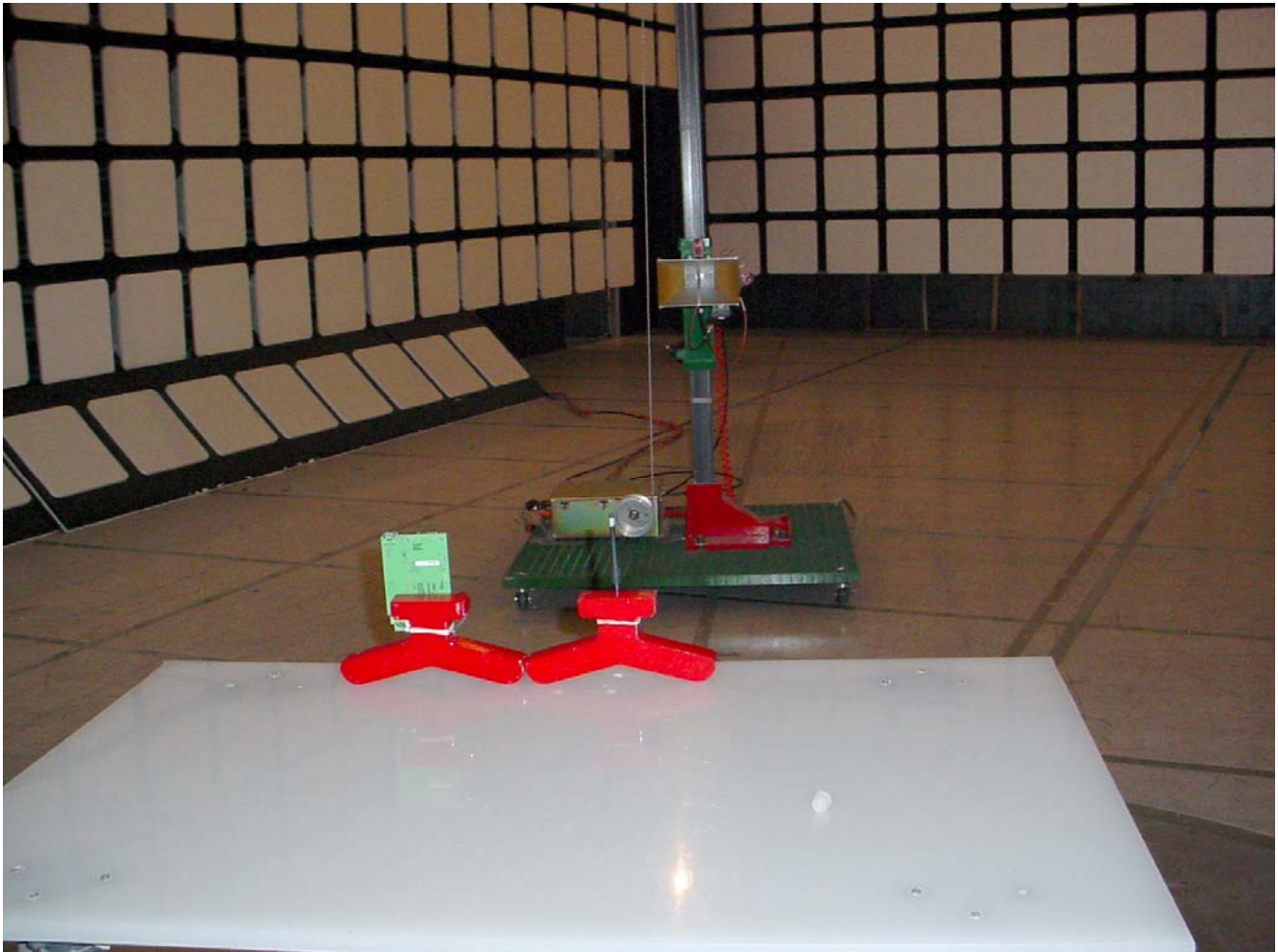
Radiated Emissions @ 3 Meters EUT with 2 dBi Rubber Ducky Antenna
