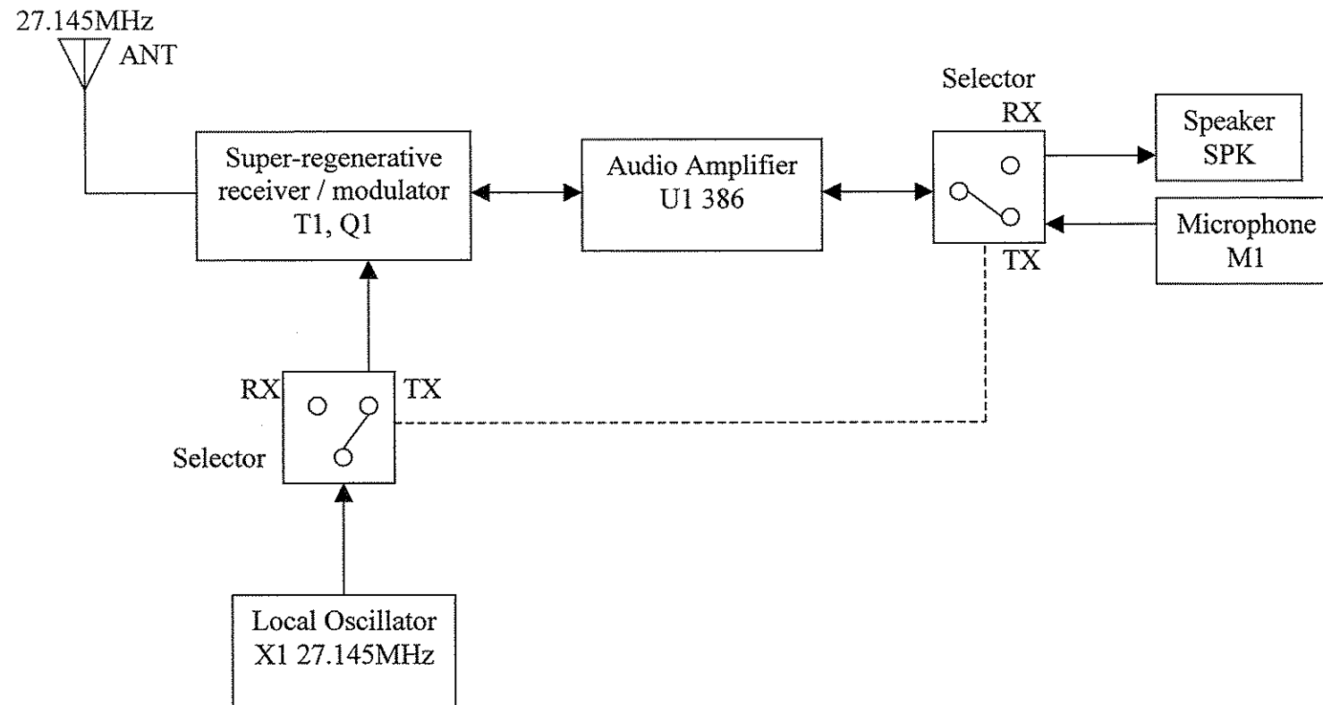
Block Diagram of #61075.
