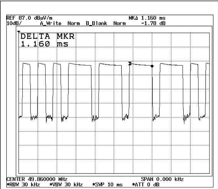
Duty Cycle 2
