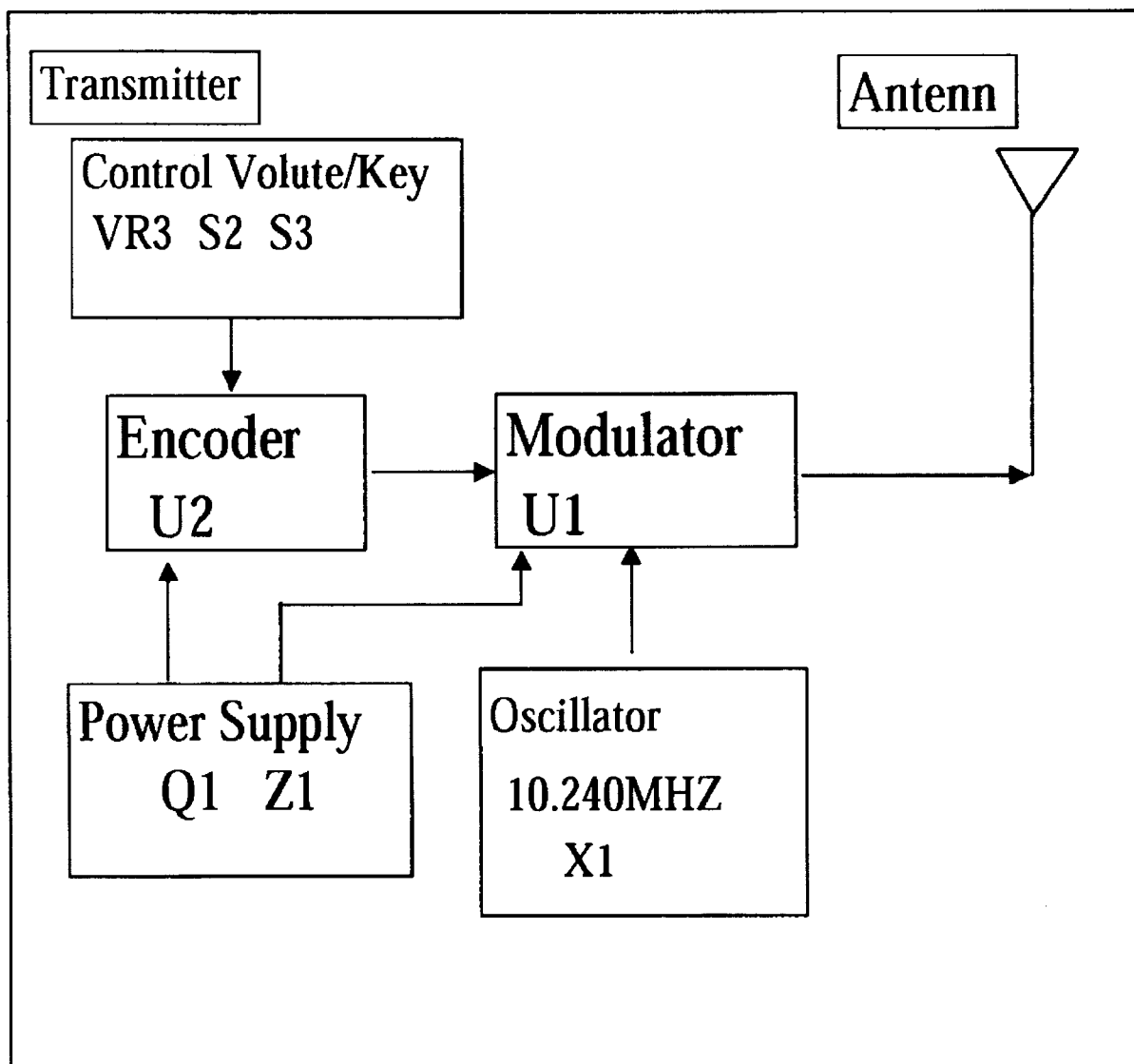
ML15106 RC Stealth Boat Bolck Diagram ( 方塊圖 )
