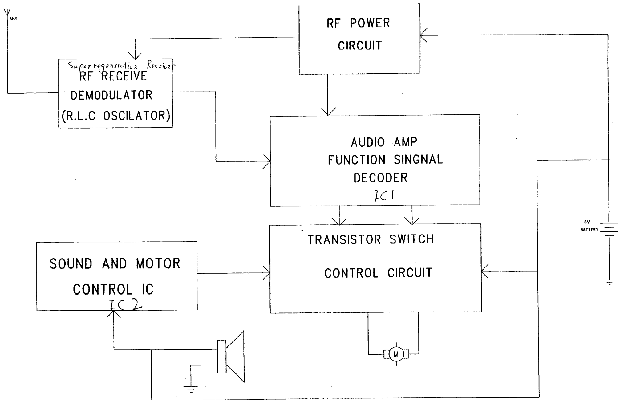
ML13971 RX BLOCK DIAGRAM
