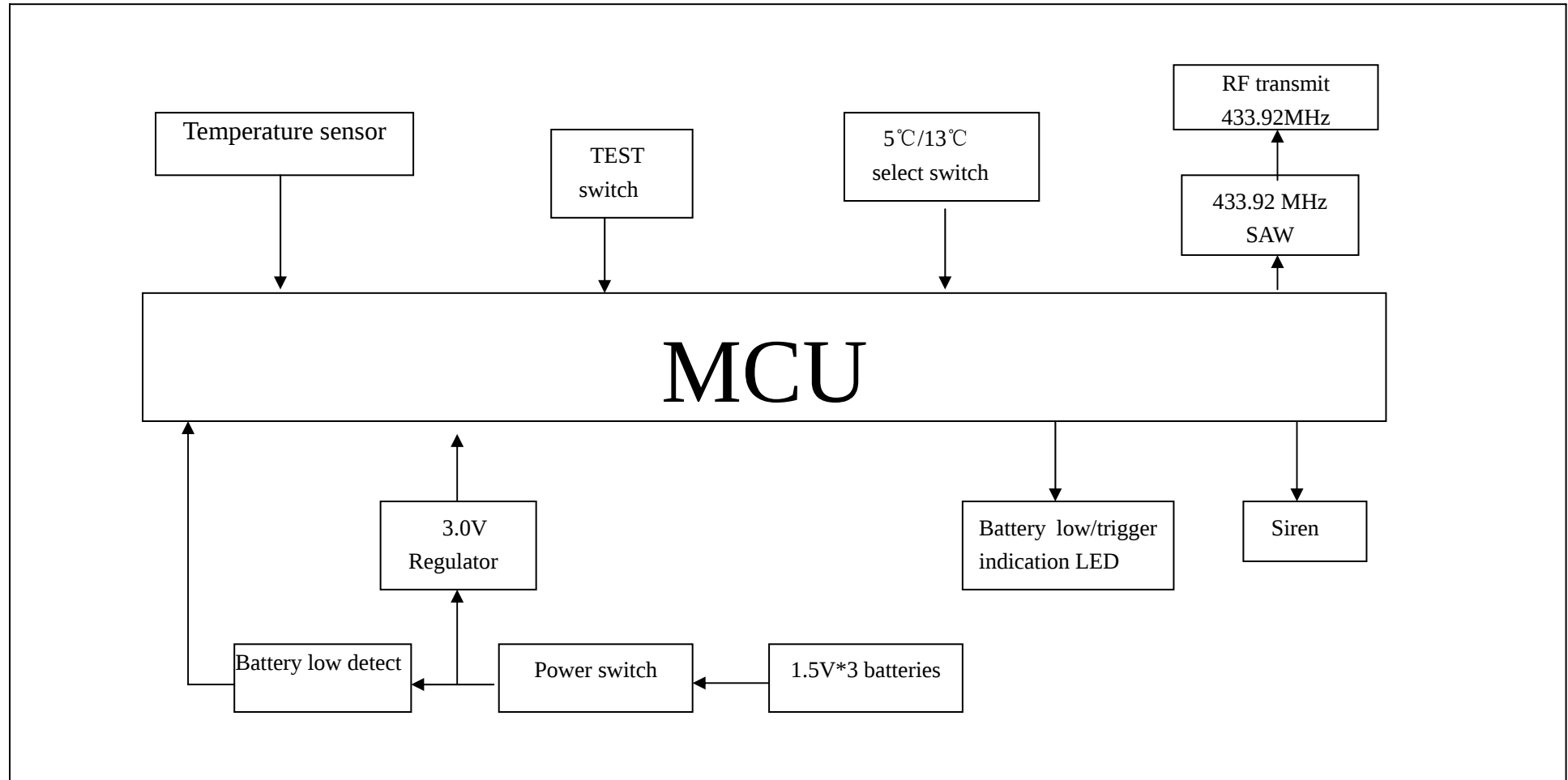
763T BLOCK DIAGRAM
