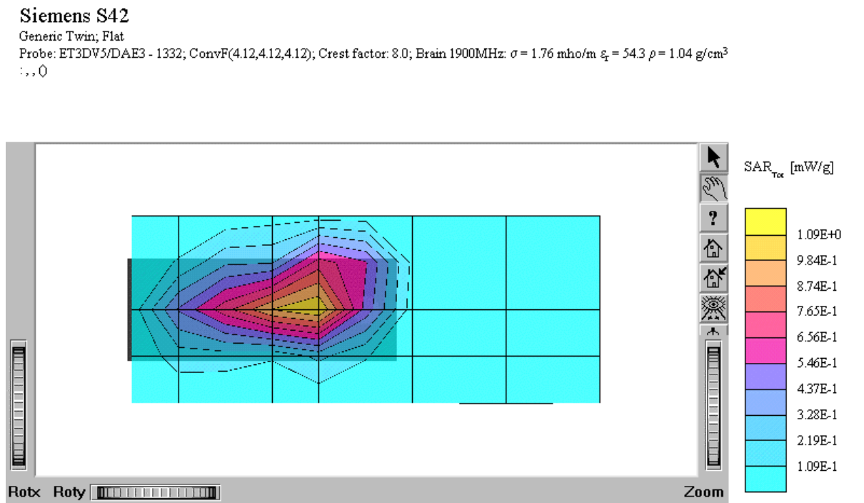
Fig. 5: SAR distribution plot with maximum local SAR value for PCS 1900 (channel 0512, hip position, the display is oriented towards to the ground. The SAR measurement is performed in the flat part of the phantom (representing the trunk of the body).)
