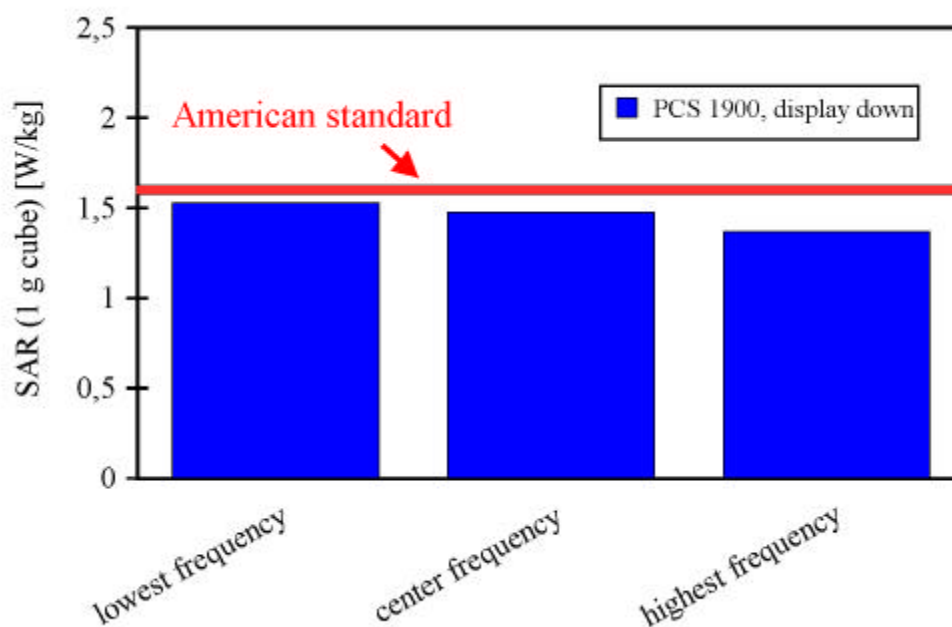
Fig. 4: The measured SAR values for PCS 1900 using the Siemens S42 in comparison to the American standard.
