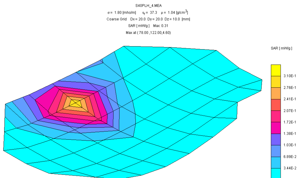
Fig. 4: SAR distribution plot with maximum local SAR value for PCS 1900 (channel 0810, left hand position).
