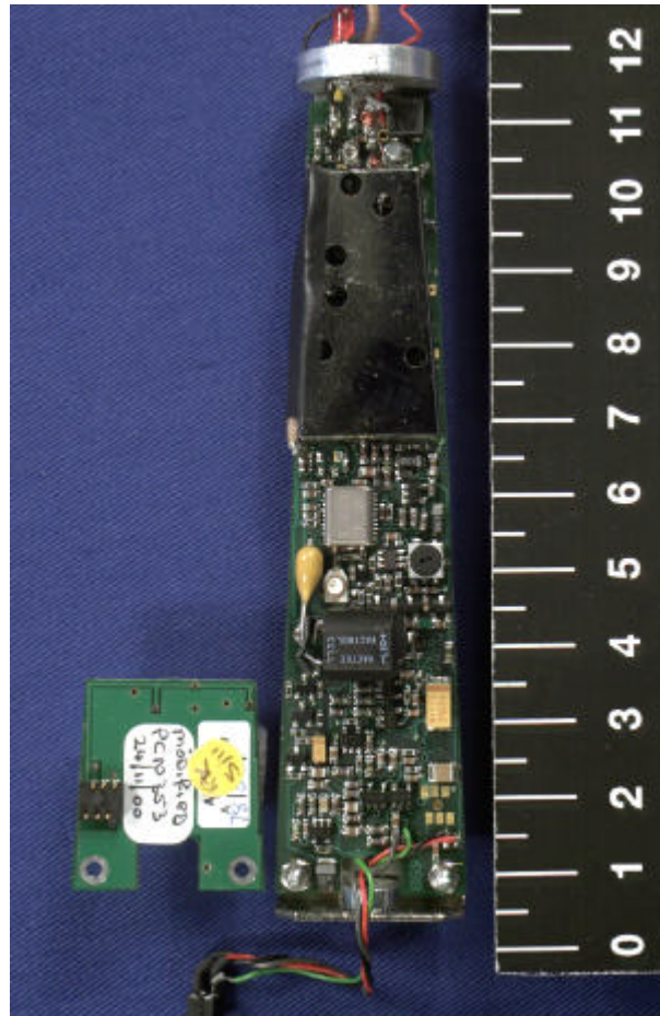
RF and Audio PCB with Comander removed
