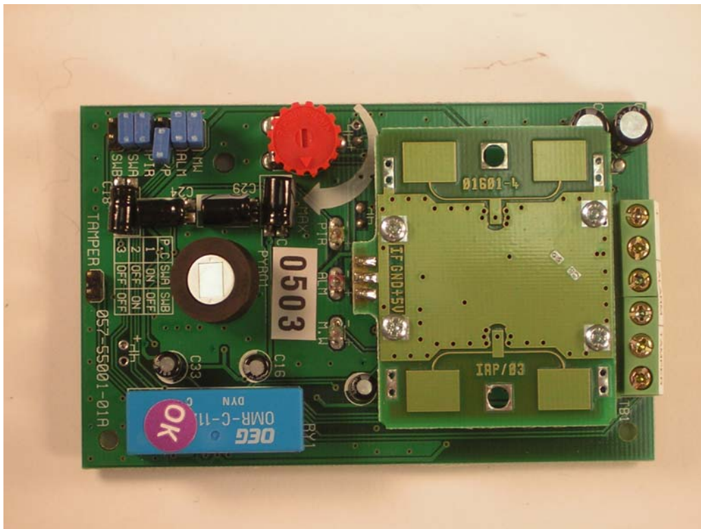
DP550 PCB top view with transmitter module installed
