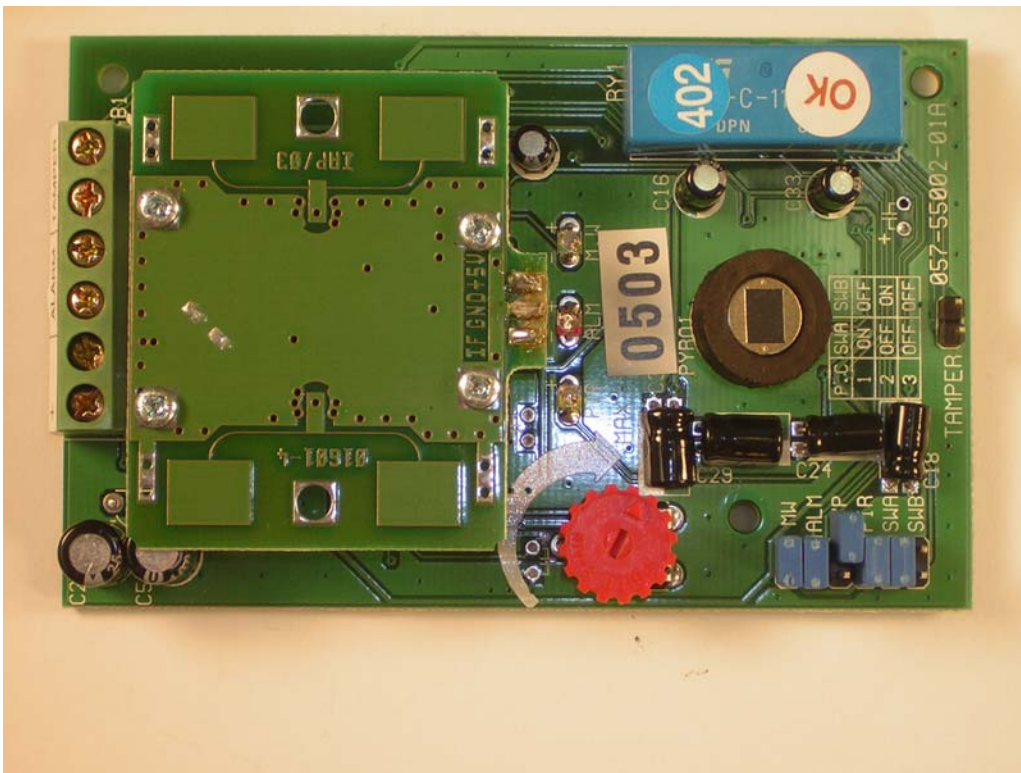
DP550P PCB top view with transmitter module installed
