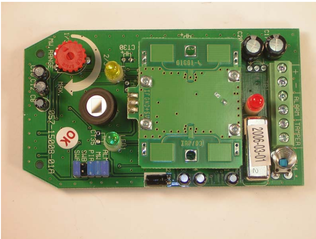
DP250 PCB top view with transmitter module installed
