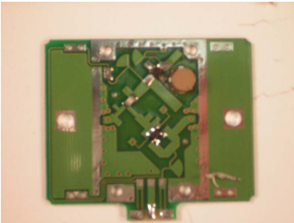
DP250, DP550, and DP550P transmitter module without plastic cover
