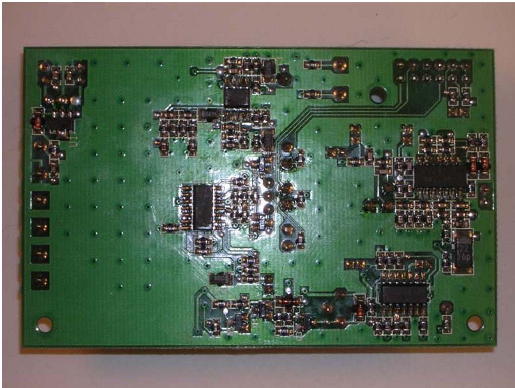
DP550P PCB bottom view
