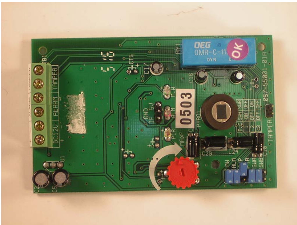
DP550 PCB top view with transmitter module removed
