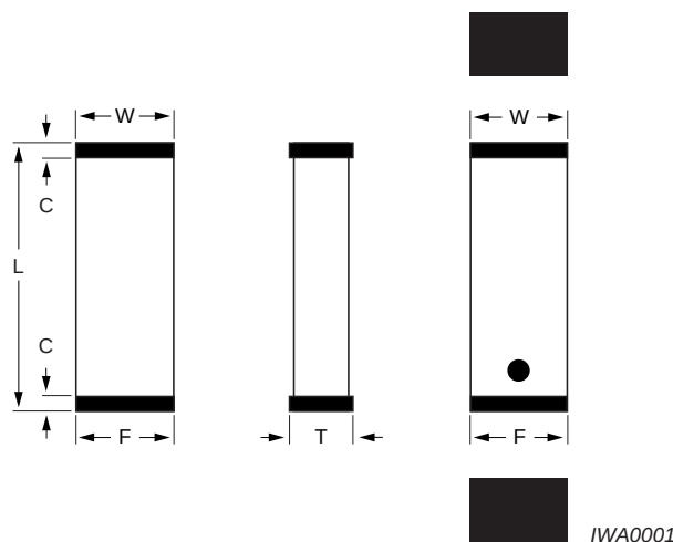
Fig.1. Component outline.
