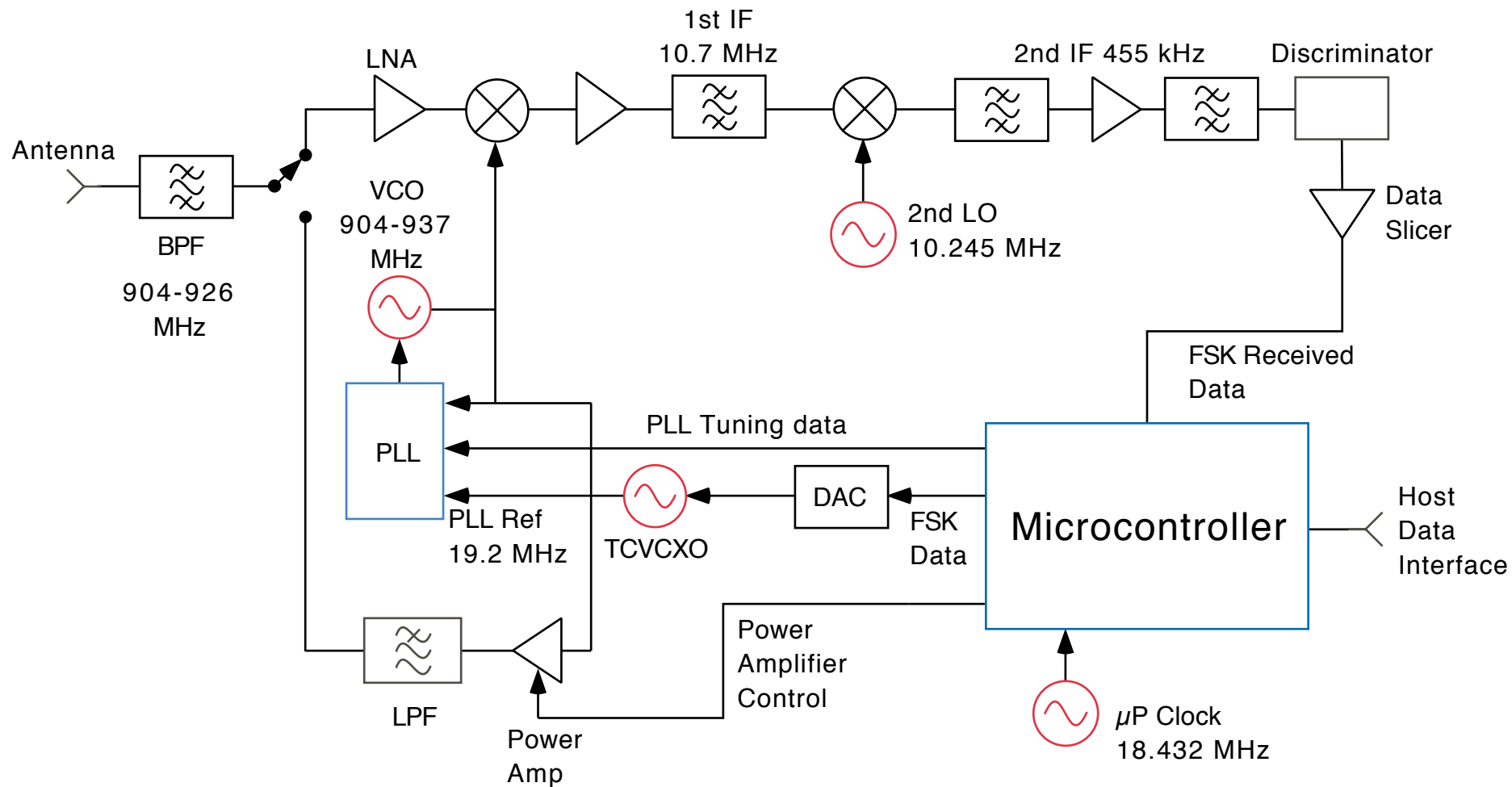
XC-900 Data Transceiver Block Diagram
