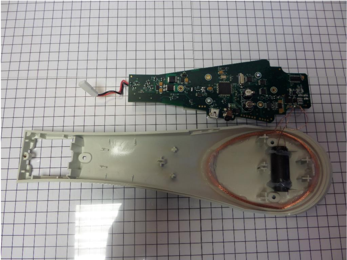
Bluetooth module with chip antenna
