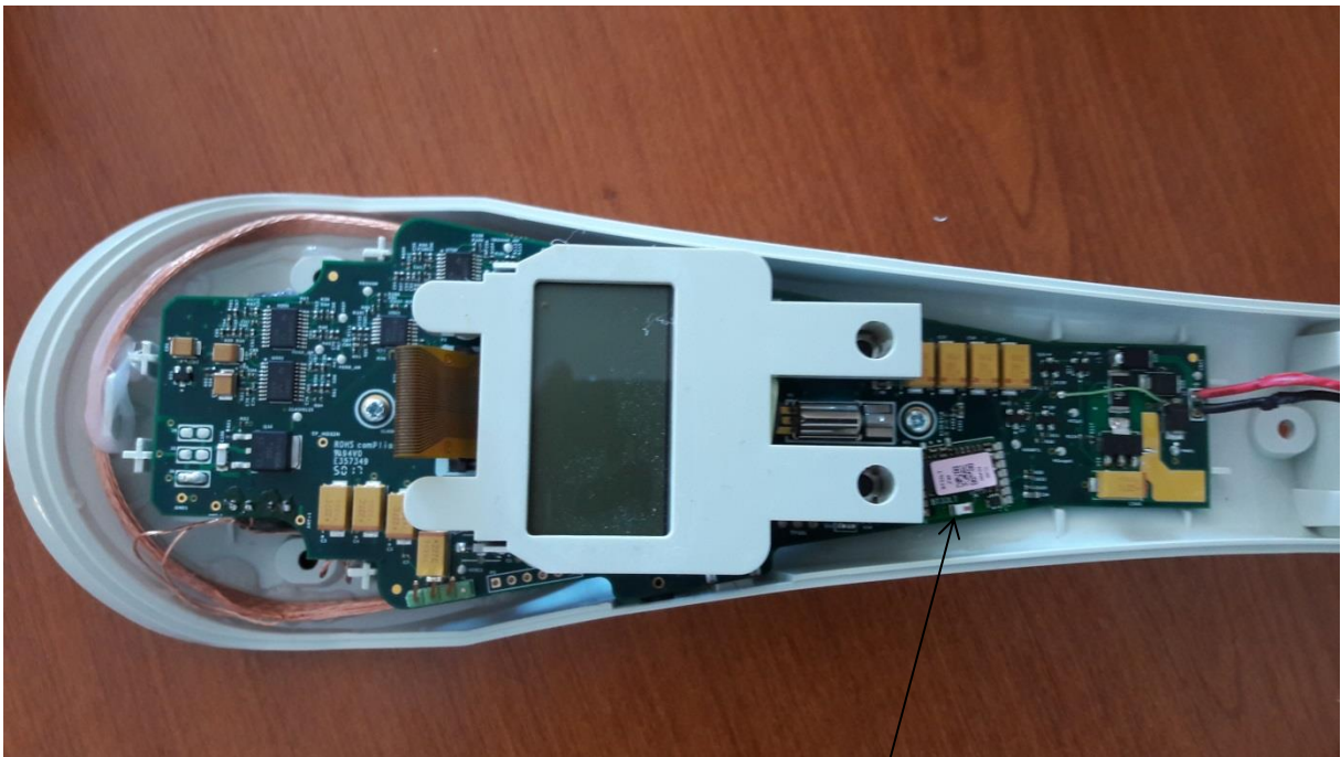
Bluetooth module with chip antenna
