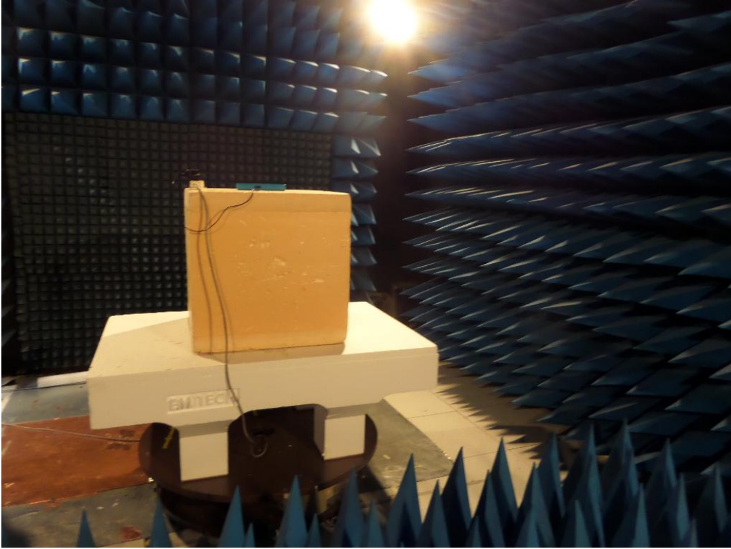
Anechoic room – RX mode
