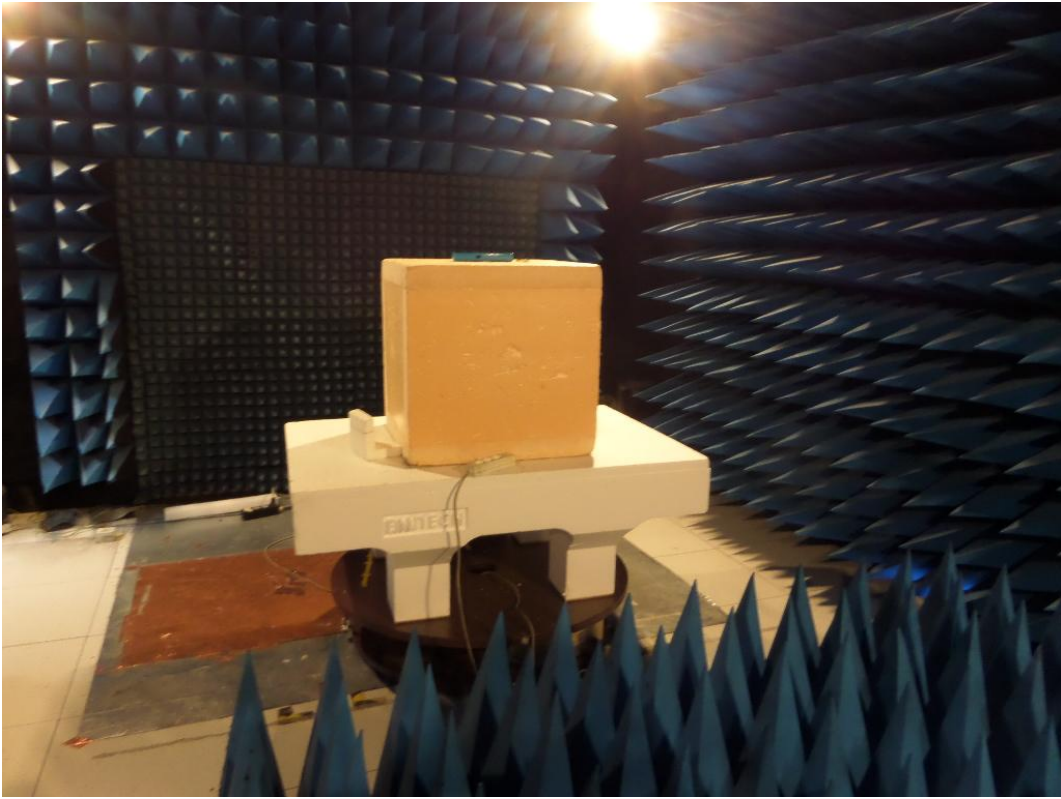
Anechoic room - TX mode
