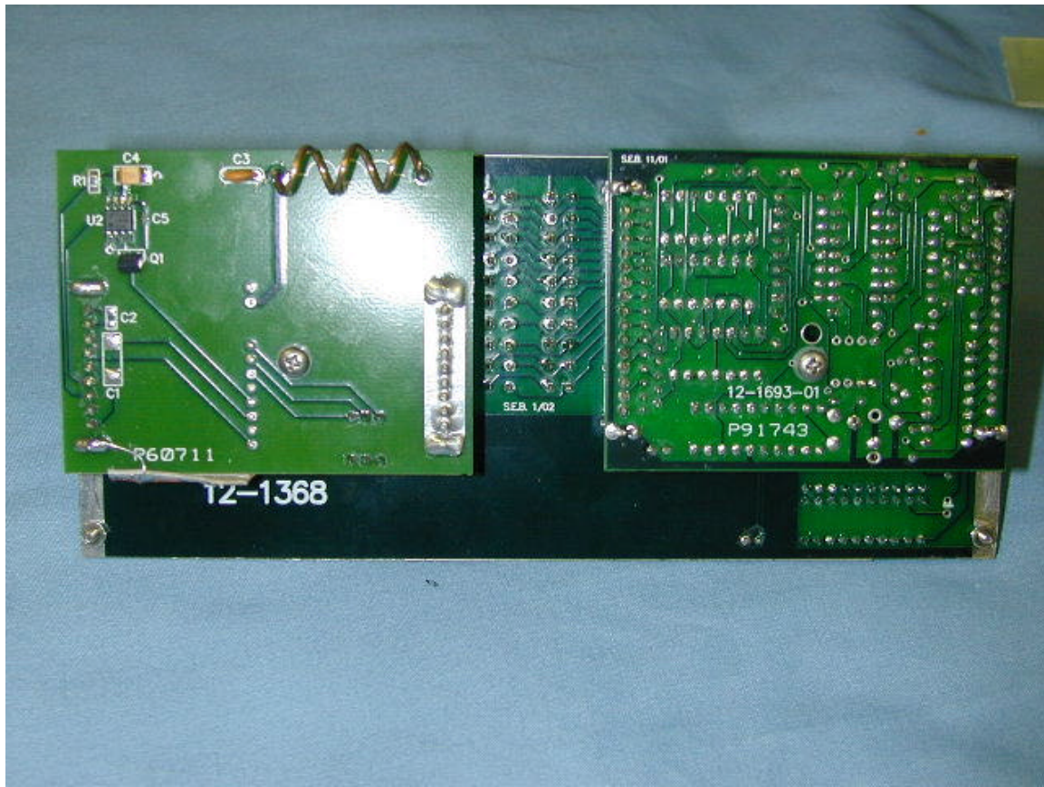
Showing mounting of Radio Board
