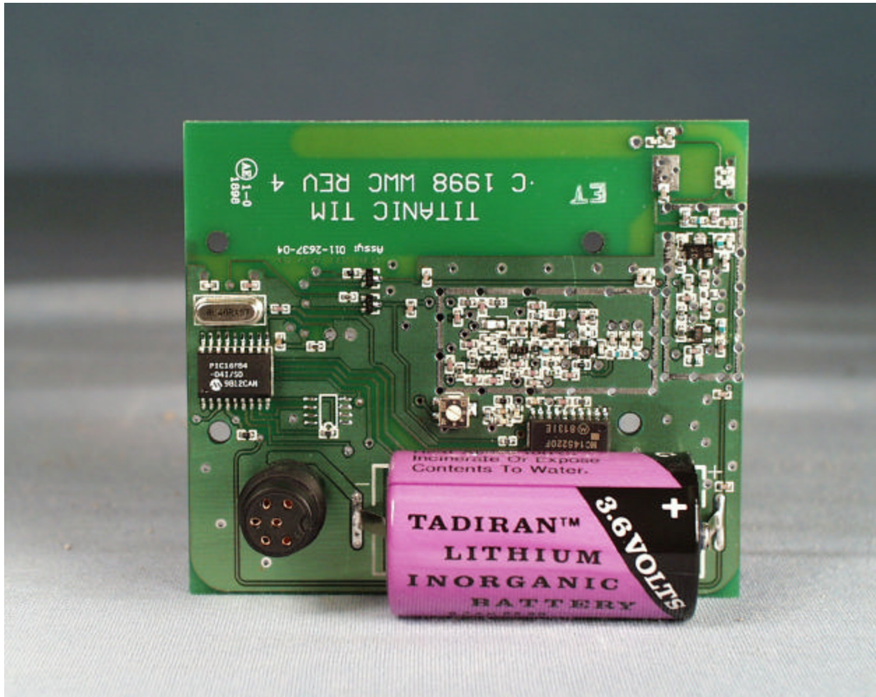
Component Side of the NQE1005 (with RF covers removed)
