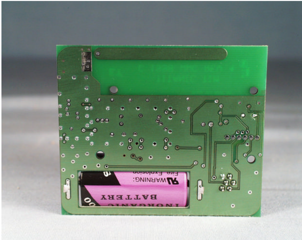
Solder Side of NQE1005
