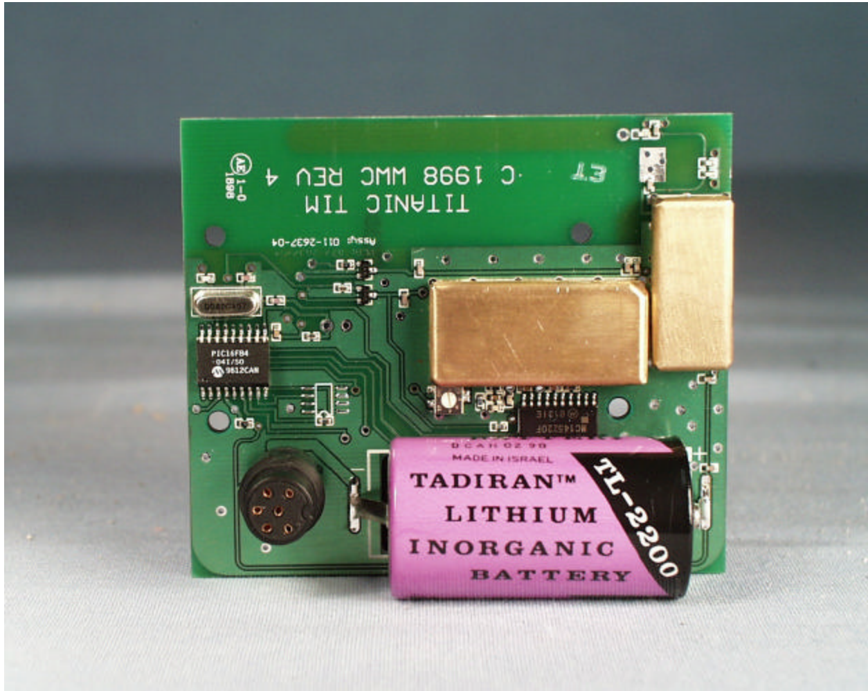
Component Side of the NQE1005 (with RF covers installed)
