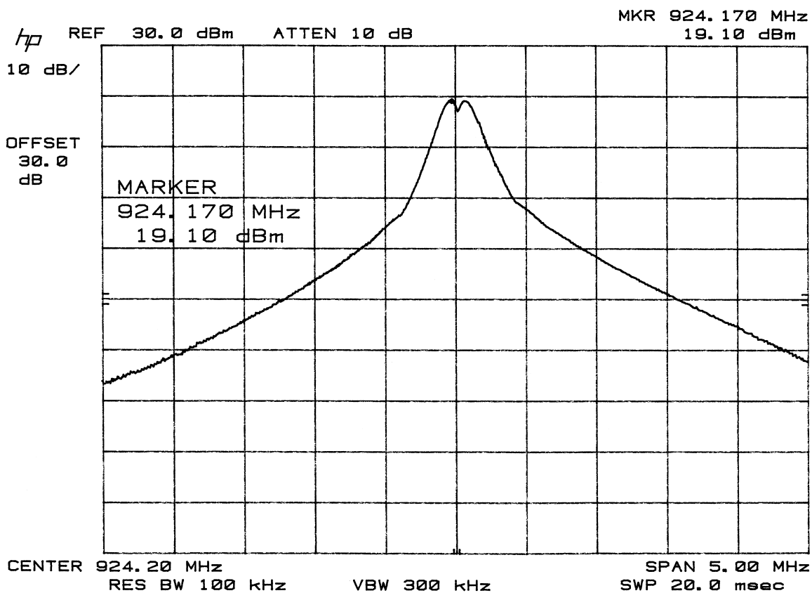
Output Power (High end of band)
