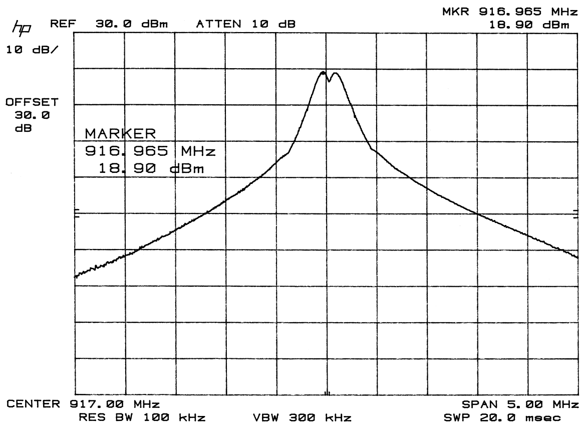
Output Power (Middle of band)
