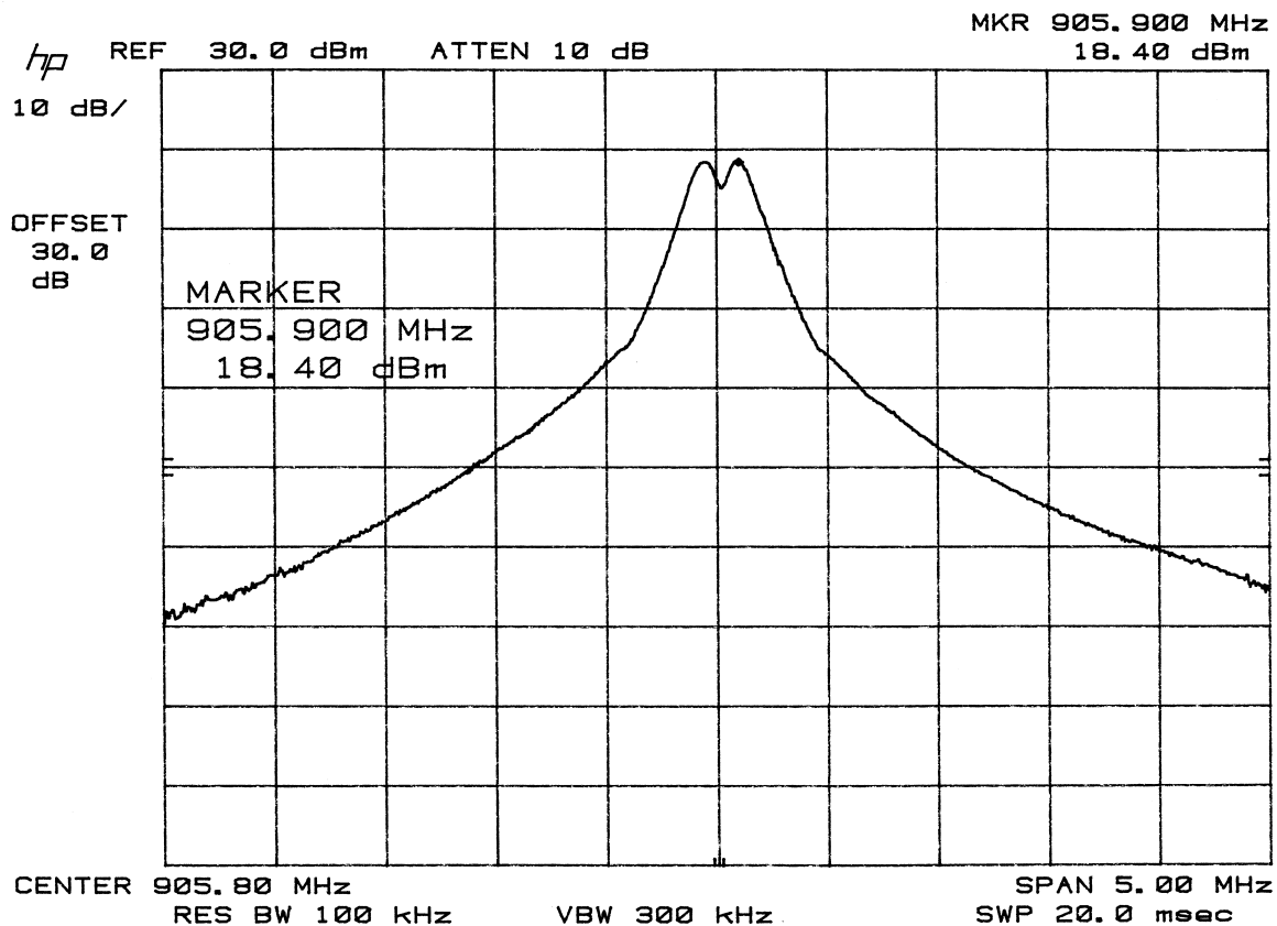
Output Power (Low end of band)
