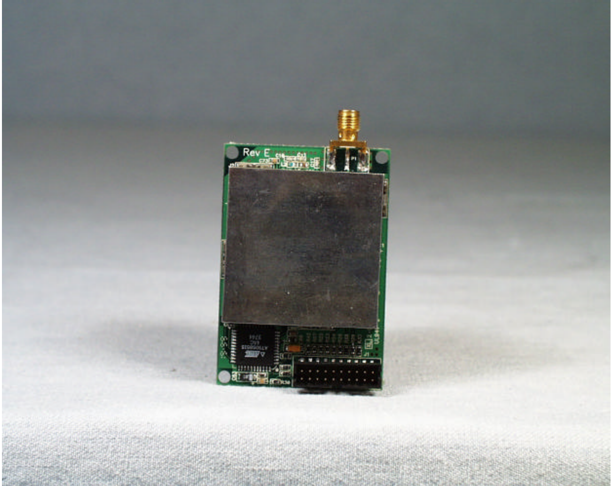
Back View of the Radio Board (with RF Can Installed)
