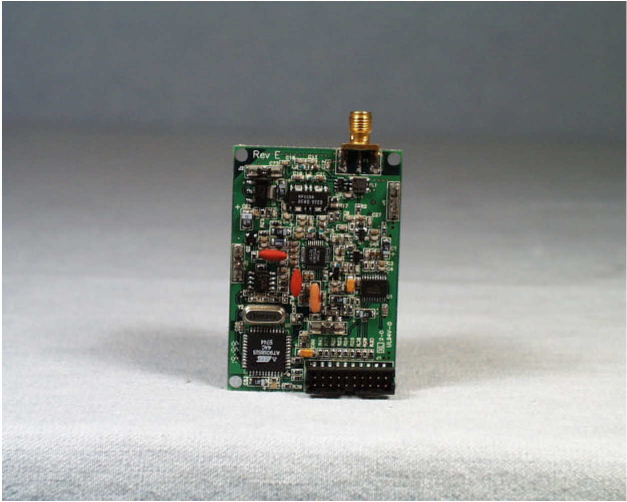
Back View of the Radio Board (with RF Can Removed)
