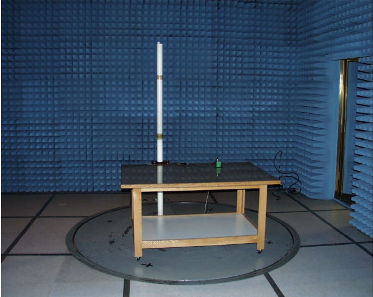
Worst case radiated emissions (Omni antenna)
