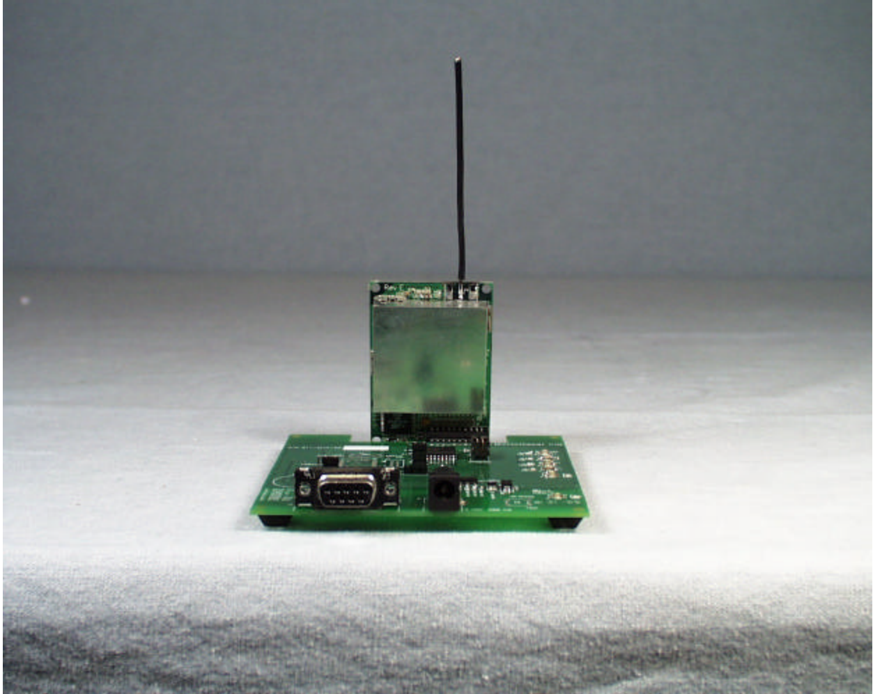
Back View of the 900 \mu Hopper and Interface Board
