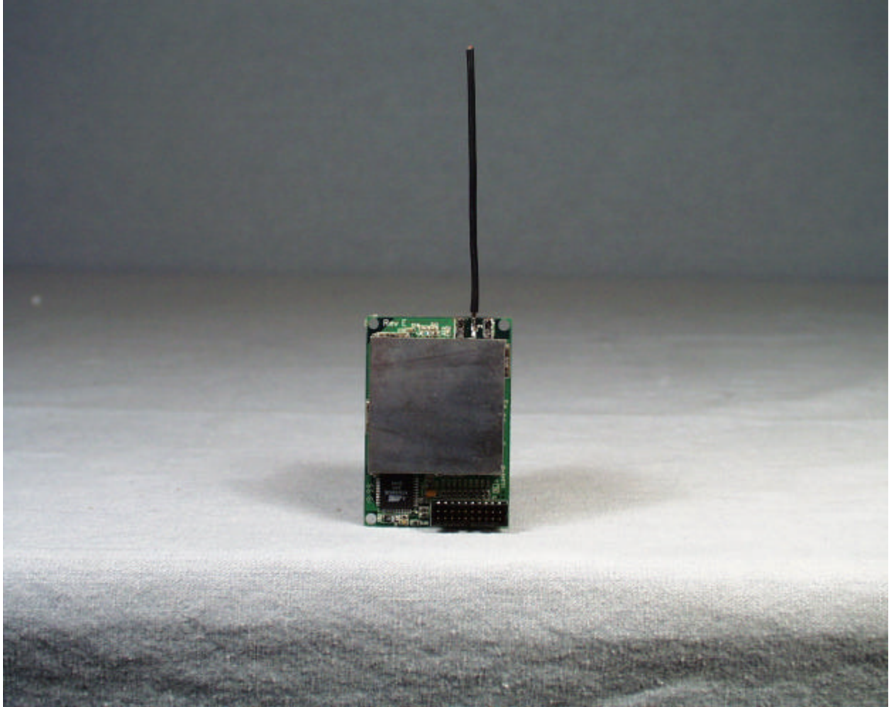
Back View of the 900 \mu Hopper (Dipole Antenna)
