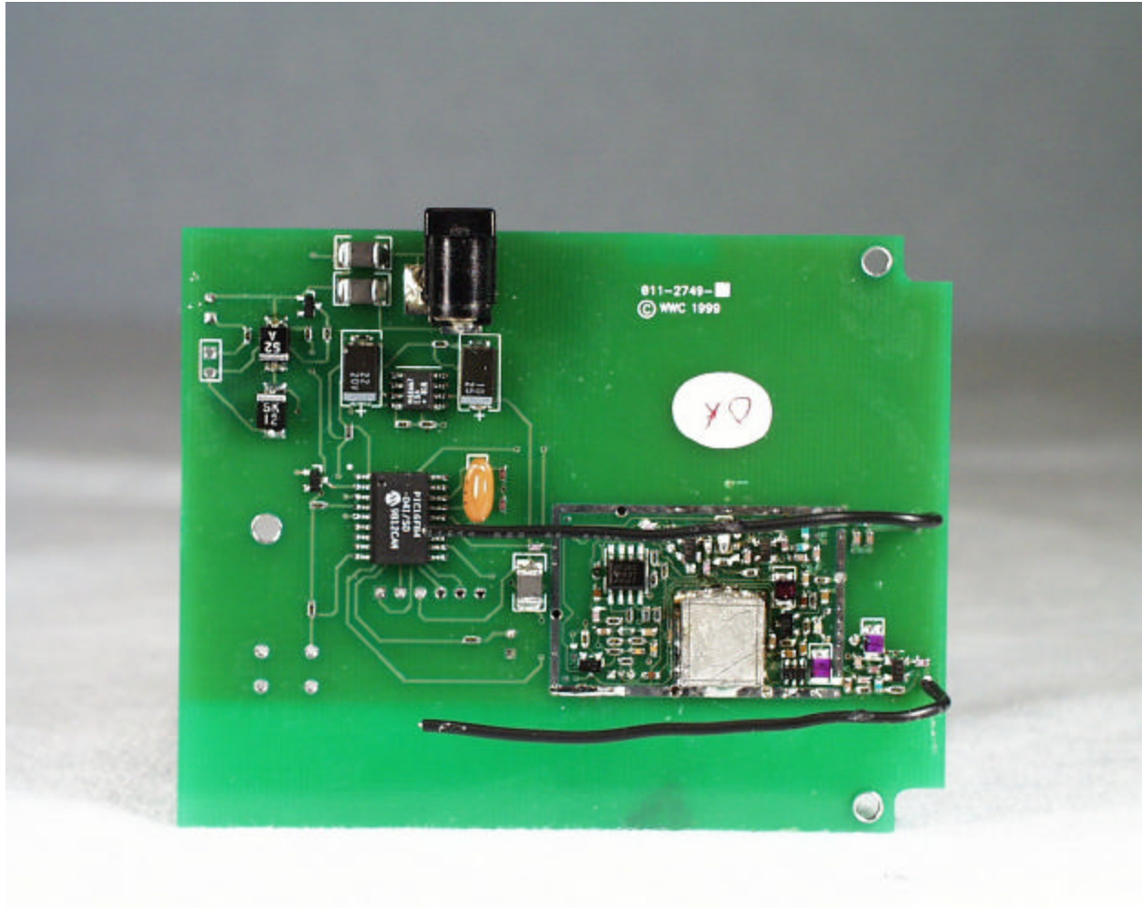
Component side of the 900 REPEATER
