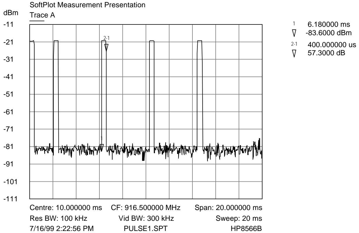
Pulse Train Plot (20 msec)
