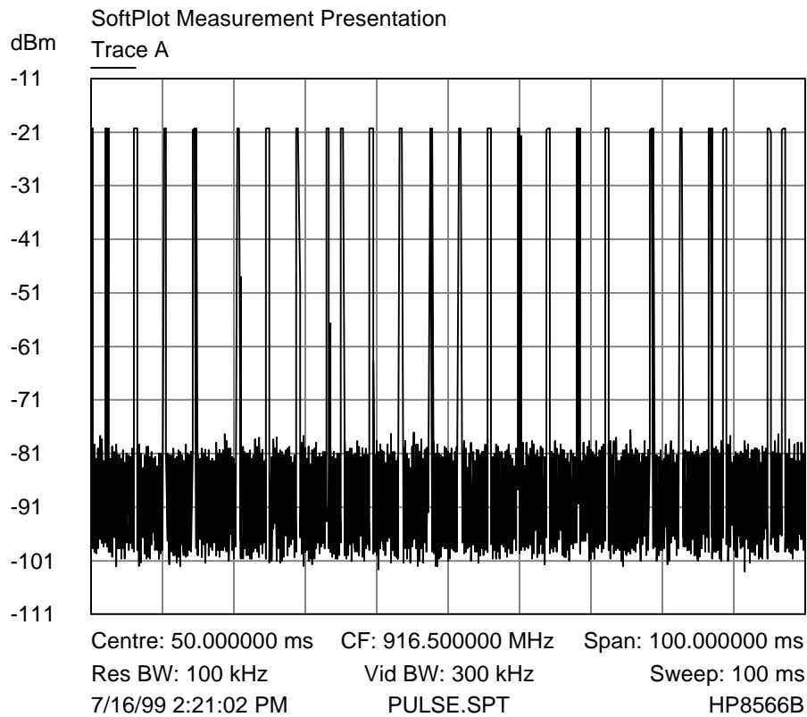
Pulse Train Plot (100 msec)
