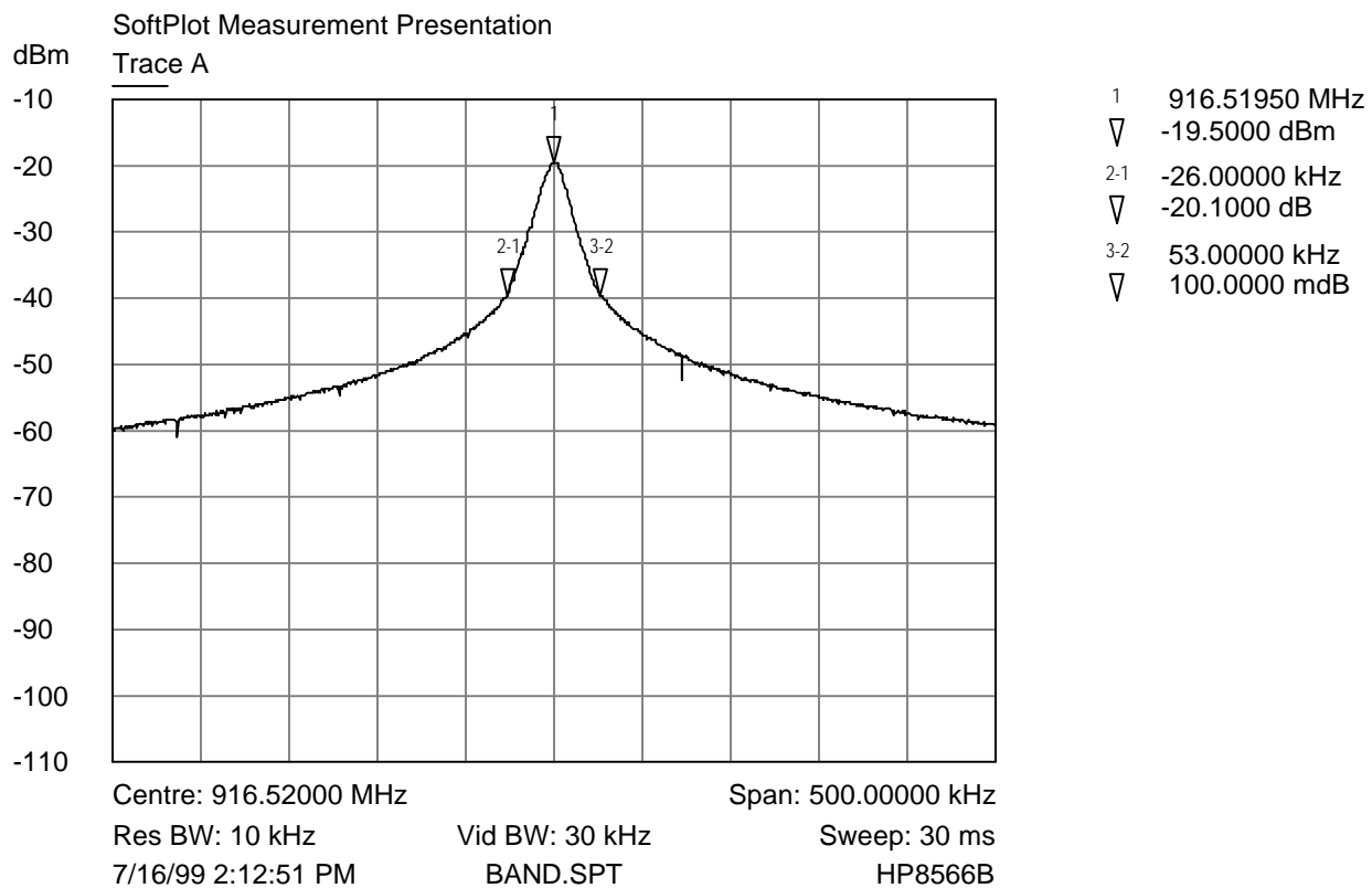
Emission Bandwidth Plot
