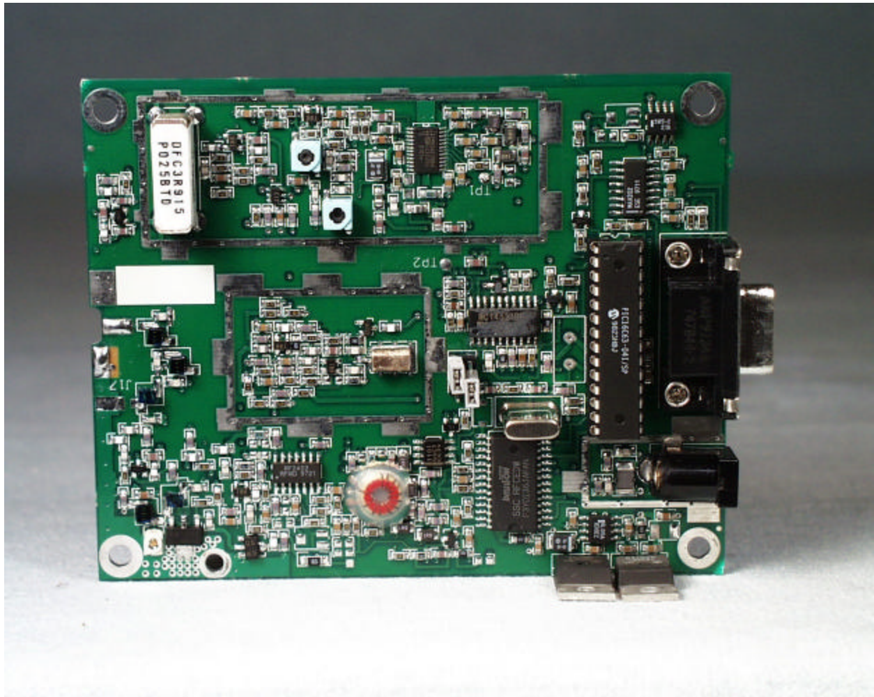
Component side of the board (with RF cans removed)
