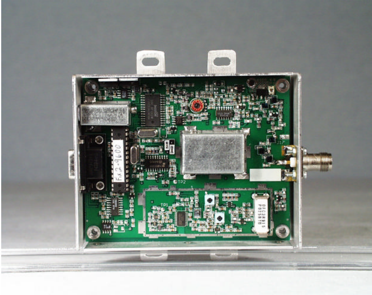
Inside View (with RF cans installed)
