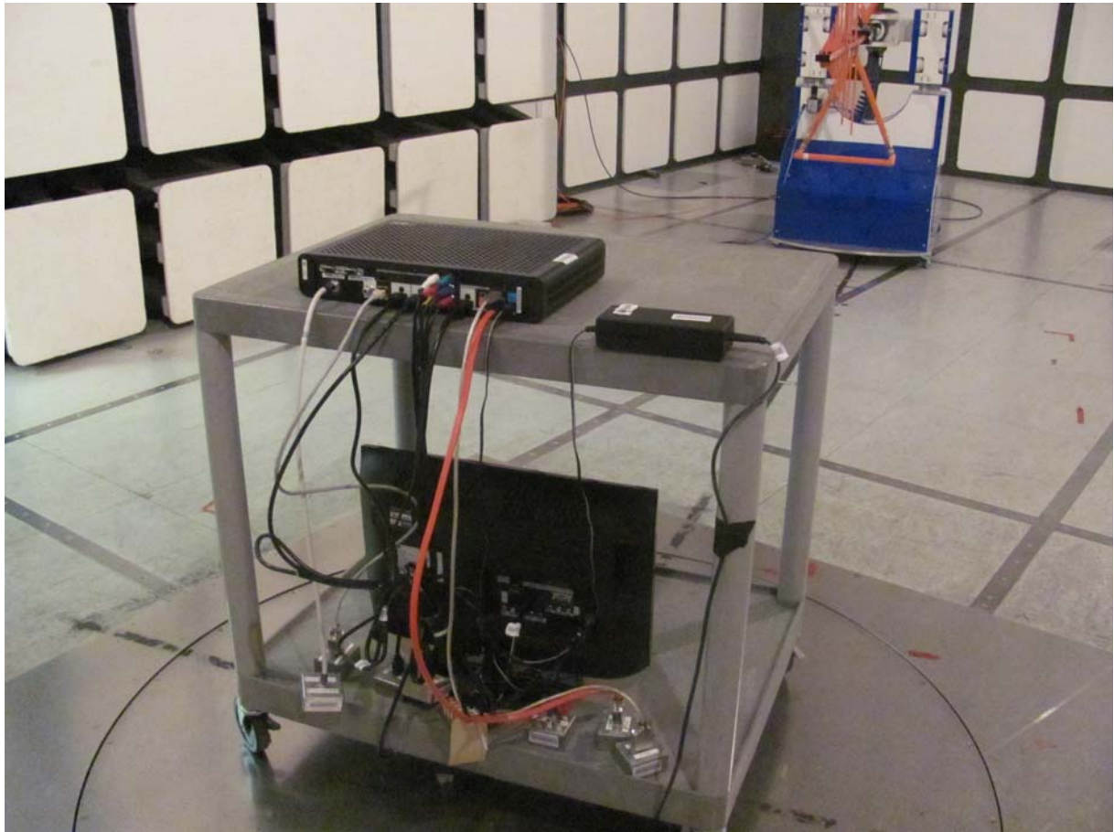
30MHz-1GHz Radiated Emissions
