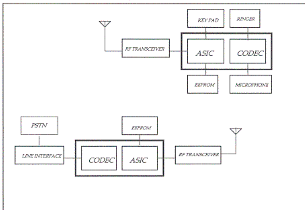
SST-911 system Architecture
