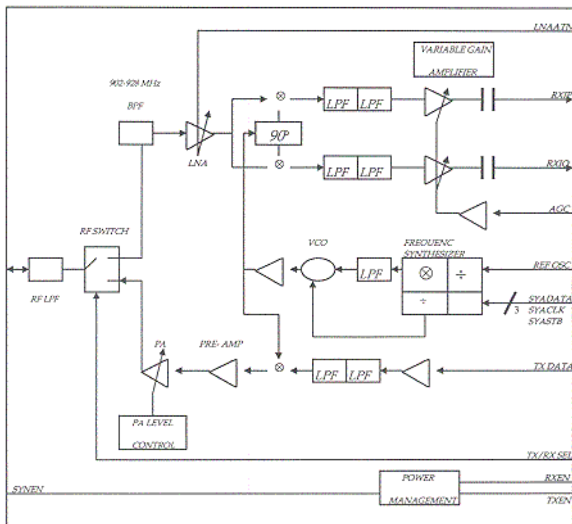
RF Block Diagram
