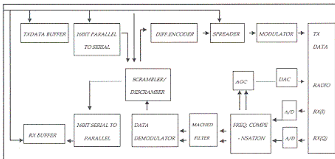
DCT Spread Spectrum Engine Block Diagram
