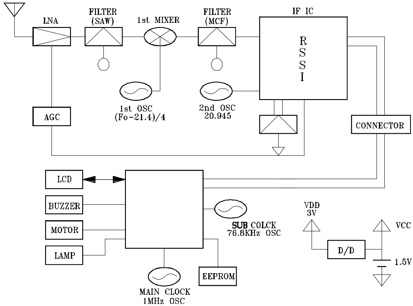
*DP-905 LOGIC/RF PART BLOCK DIAGRAM.
