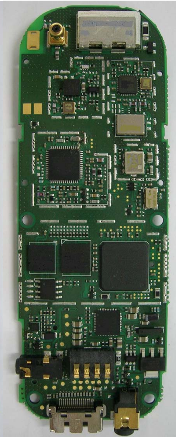
Rear View (Shields Removed)
