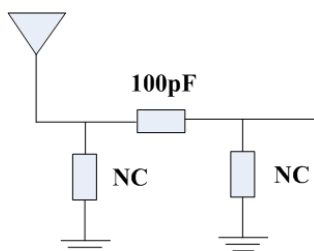
\pi Matching
