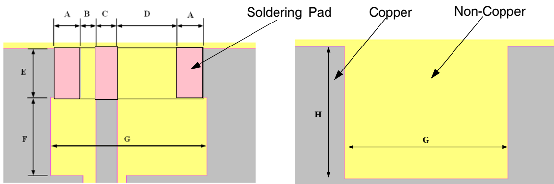
Top Layout
