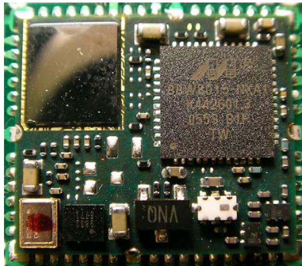
WLAN Module without Shield
