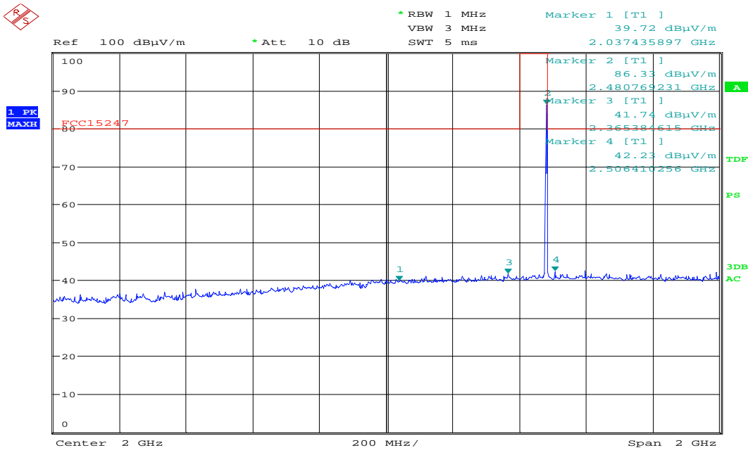
Radiated spurious emissions, VP, 1 - 3GHz, ch2480MHz, PK scan
