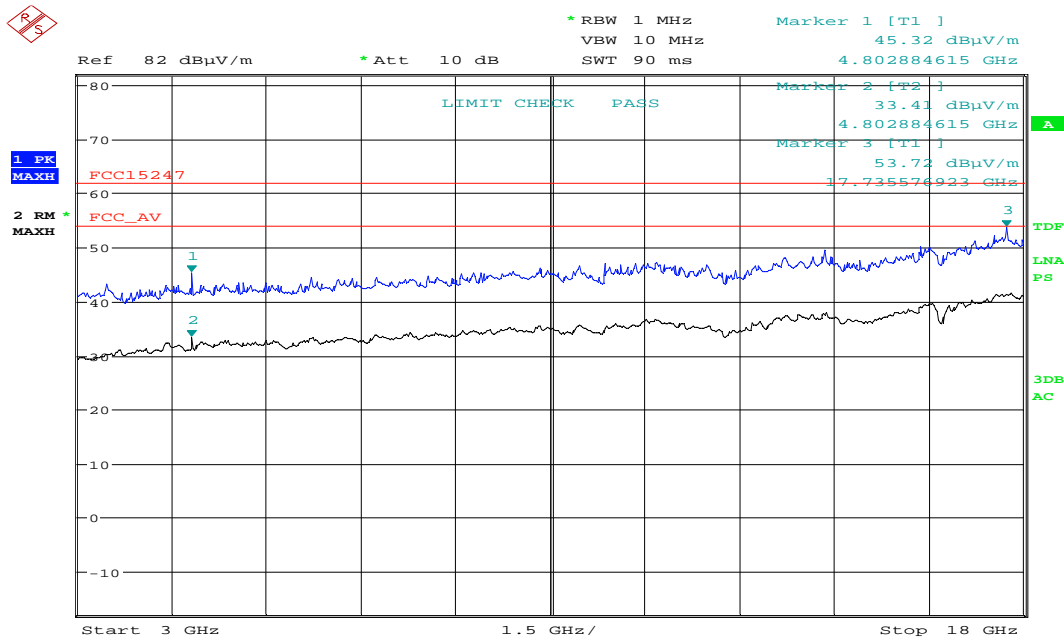
Radiated spurious emissions, VP, 3 - 18GHz, ch2402MHz, PK scan
