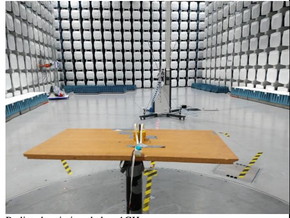
Radiated emissions below 1GHz
