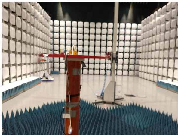
Radiated emissions > 1GHz, XZ plane
