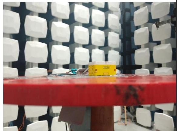
Radiated emissions > 1GHz, XY plane
