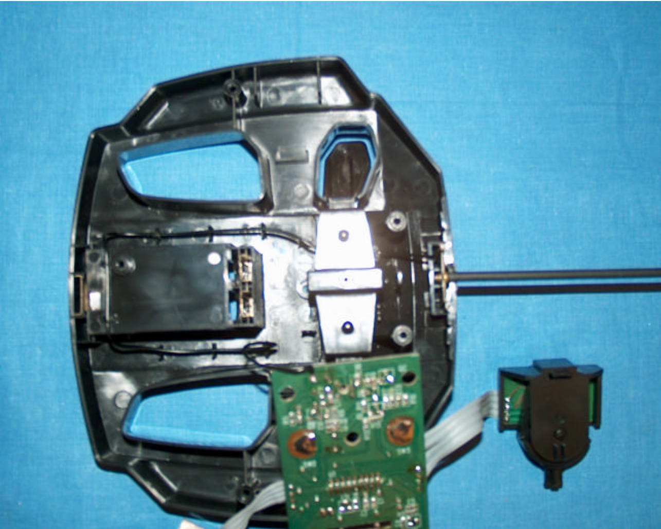
Lower cover including connection form main board to antenna (small black wire)
