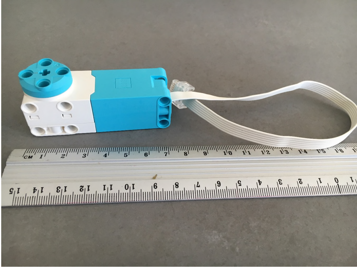
Medium motor 535894
