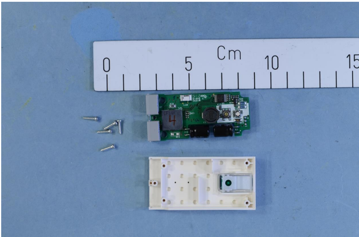
Rear side of the PCB
