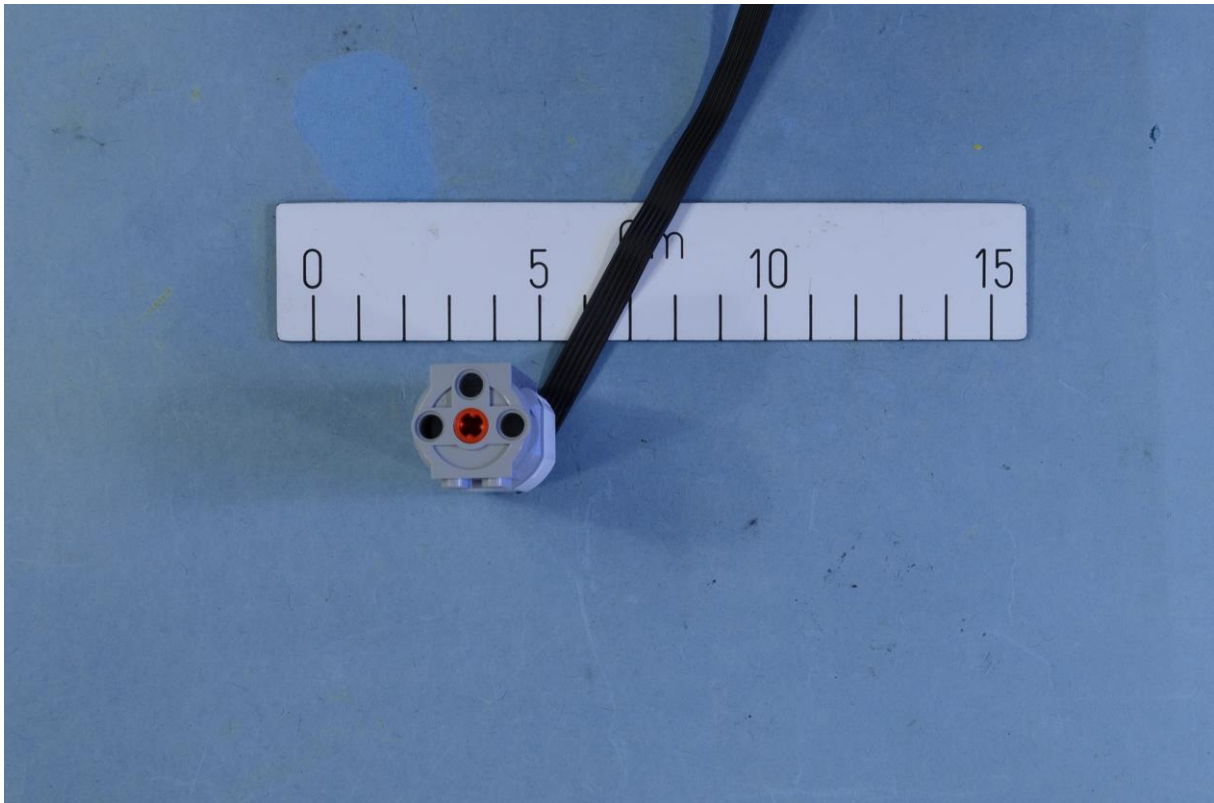
End view - 10021980 LPF2 Medium Motor
