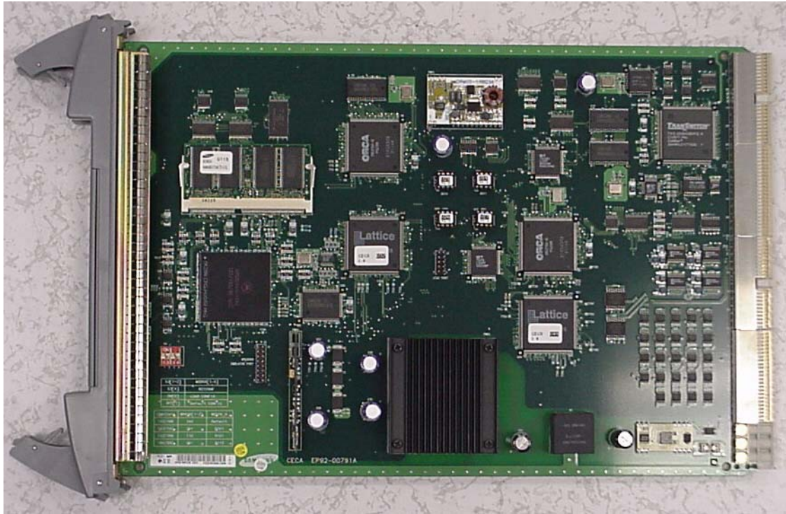
Exhibit 15 - CECA module, component side
