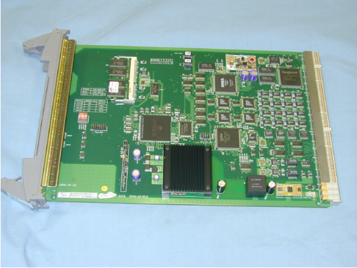
Photo 4 - BCPA Card, component side
