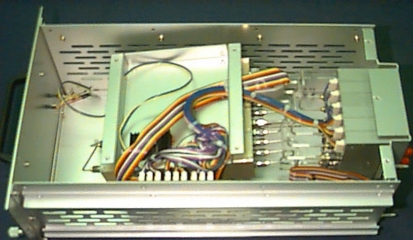
RFI/AS CARD
