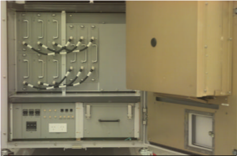
G12 : SCBS-319M-F-OPEN-LOWER
