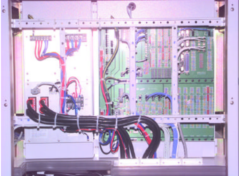
G15 : SCBS-319M-B-OPEN-UPPER
