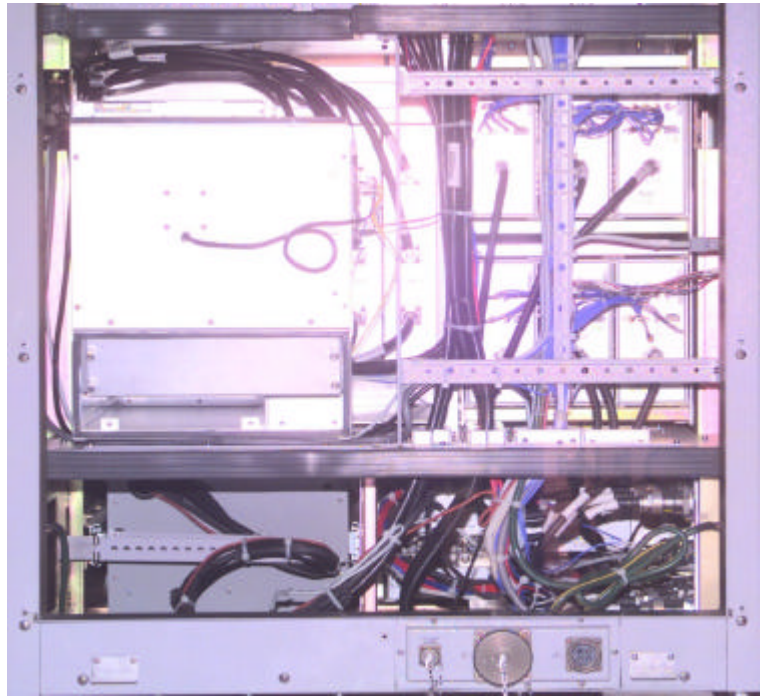
G16 : SCBS-319M-B-OPEN-LOWER
