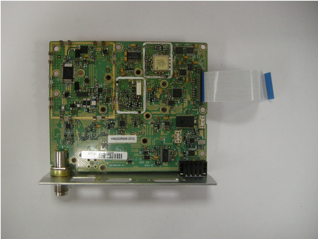
Top Side RF Board no shields
