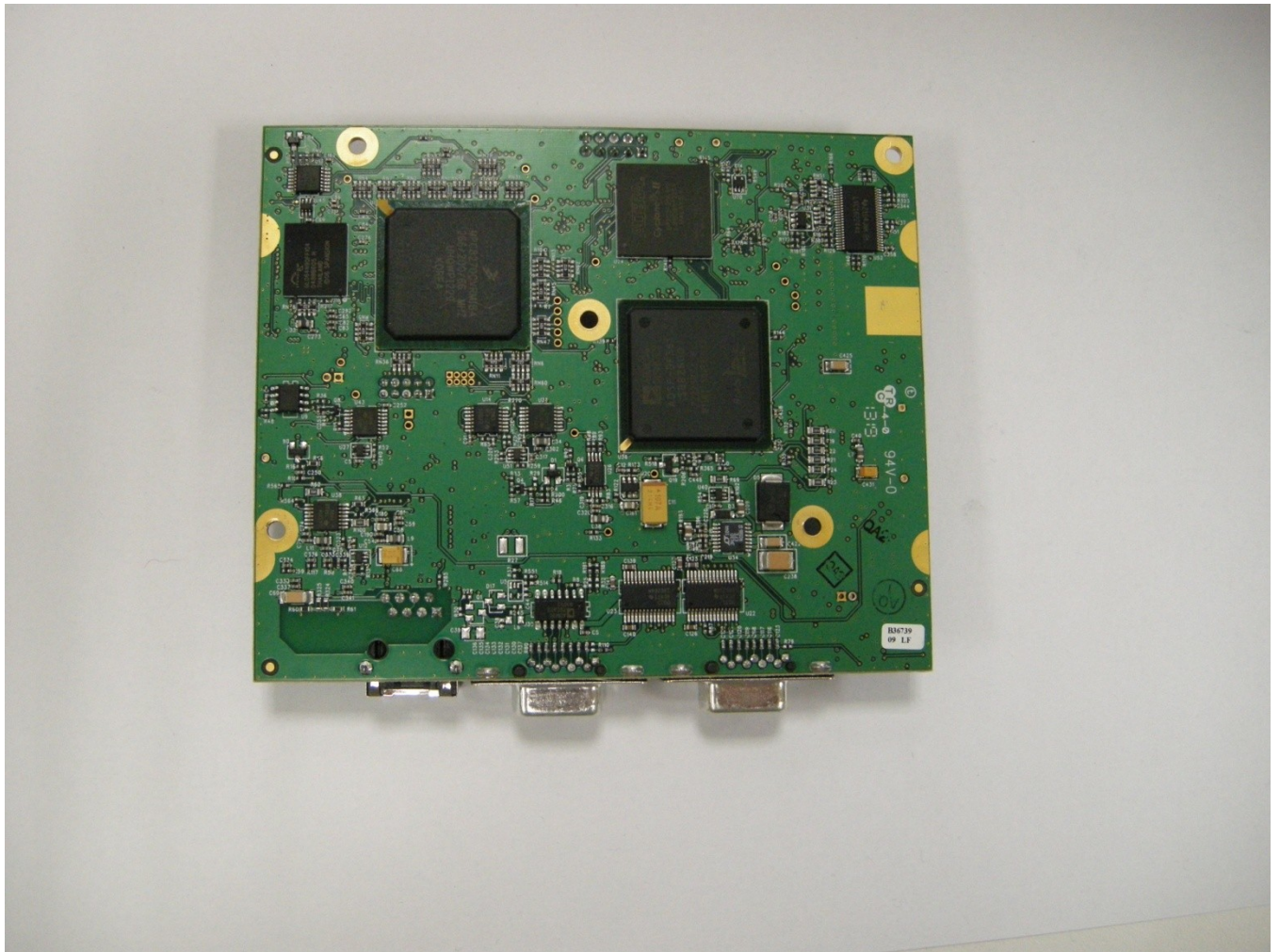
Bottom Side Modem and RF Board
