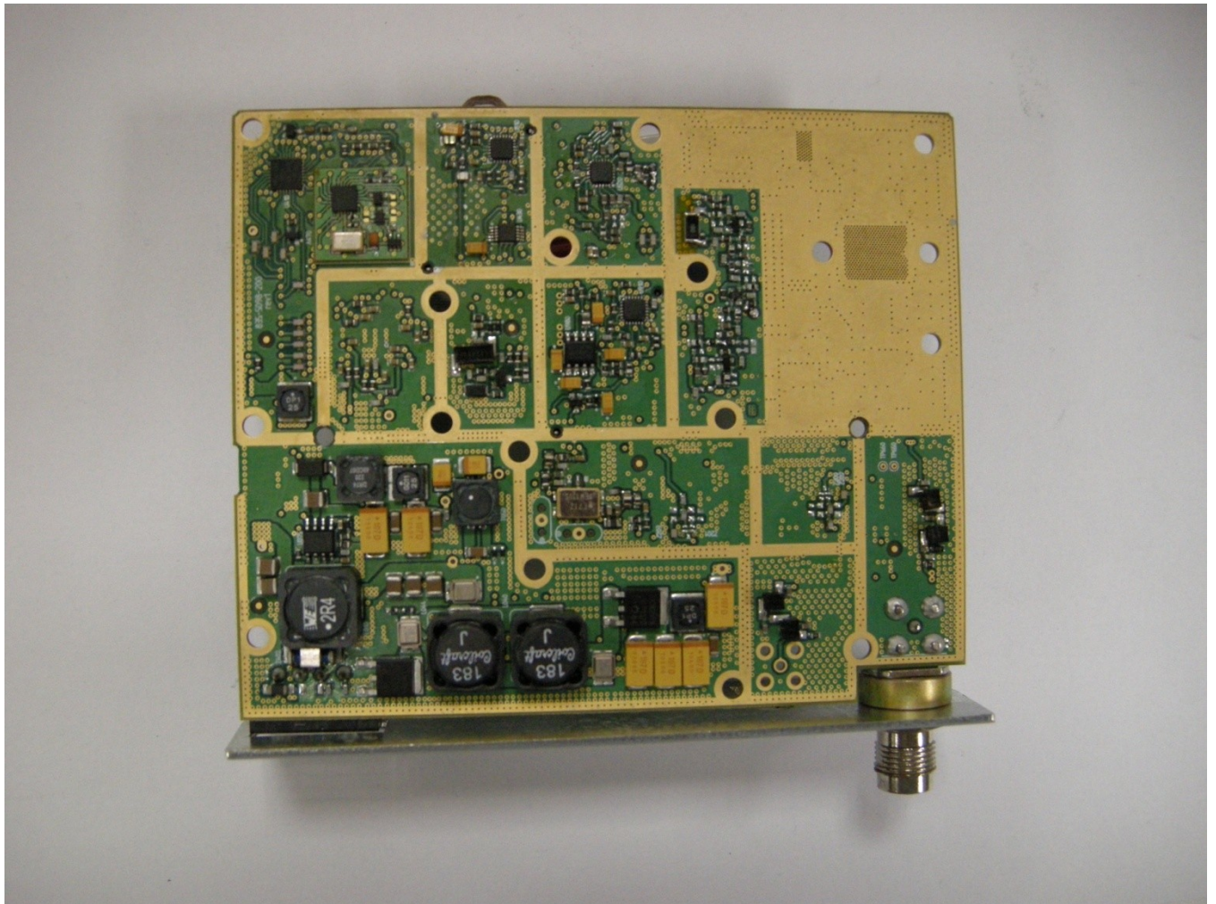
Bottom Side RF Board no shields
