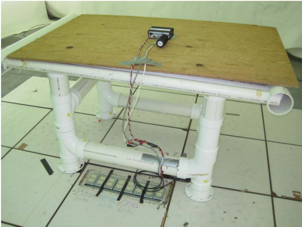
Test Setup Photo Radiated emissions
