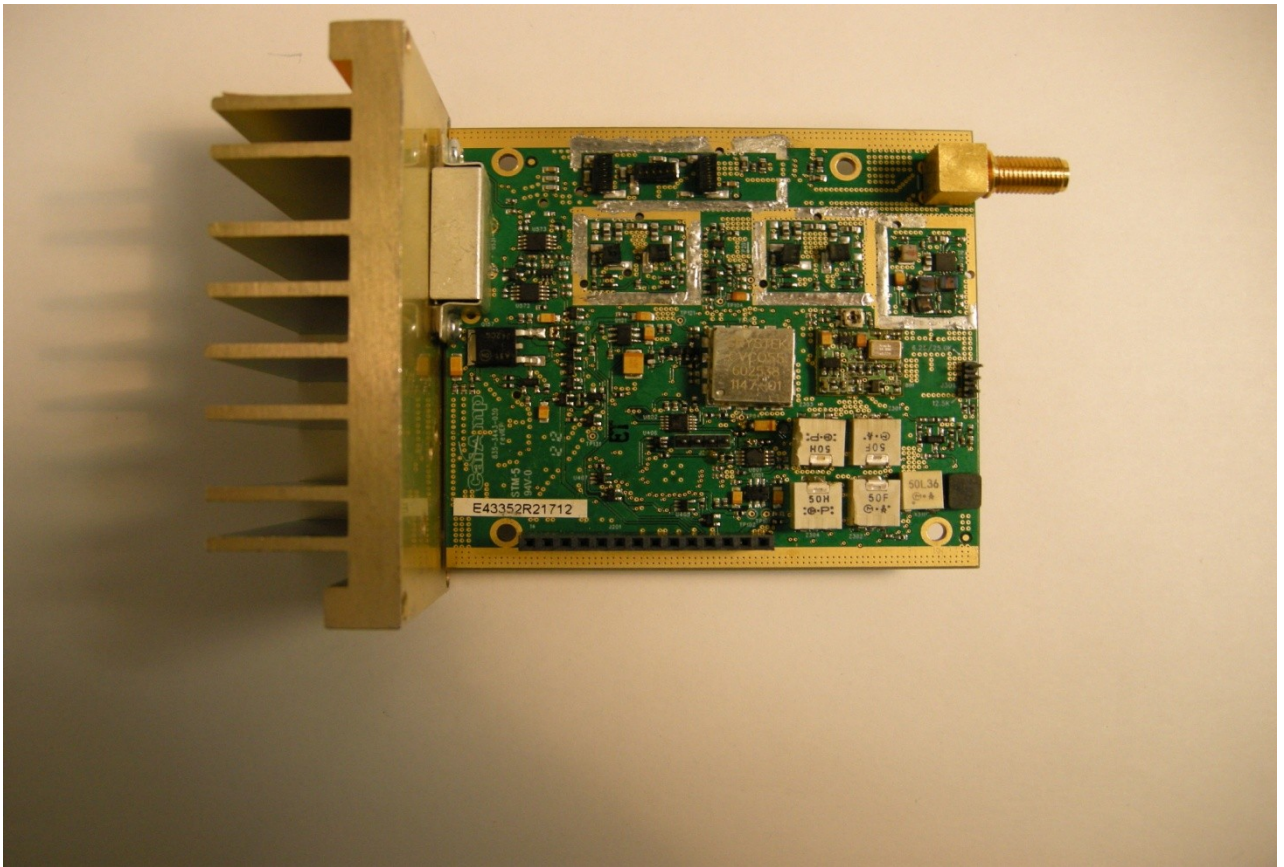
Top Side RF Board no shields
