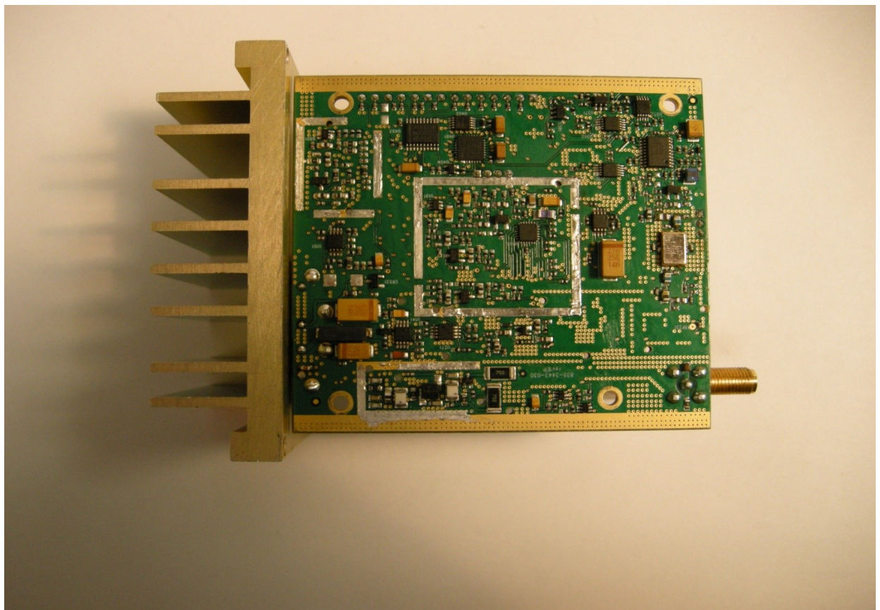
Bottom Side RF Board no shields
