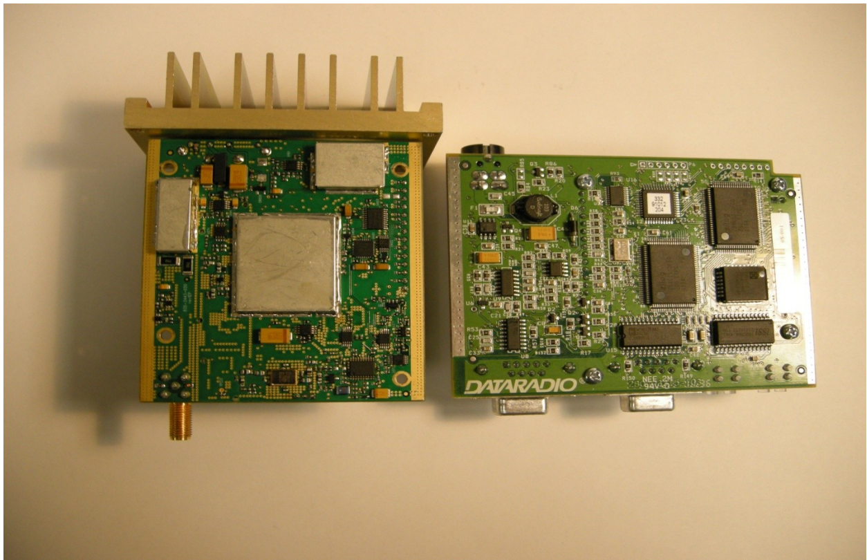
Bottom Side Modem and RF Board
