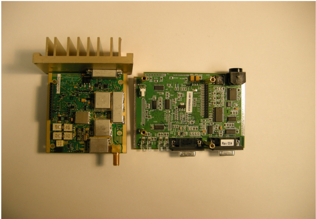
Top Side Modem and RF Board
