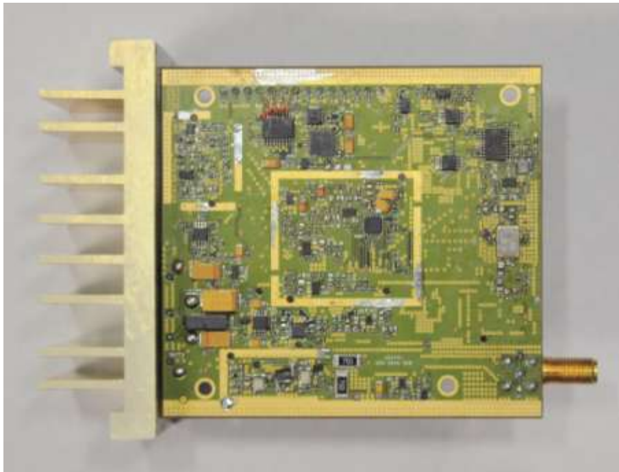
Bottom Side RF Board no shields
