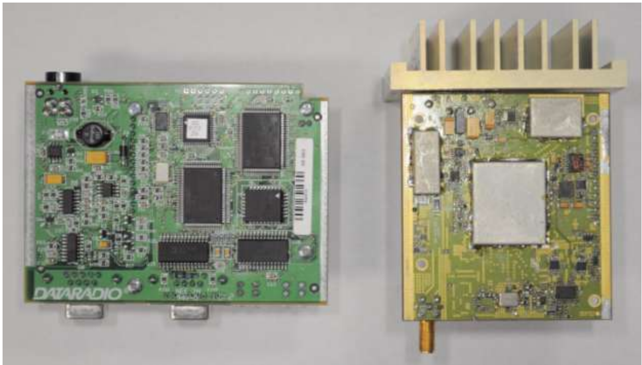
Bottom Side Modem and RF Board
