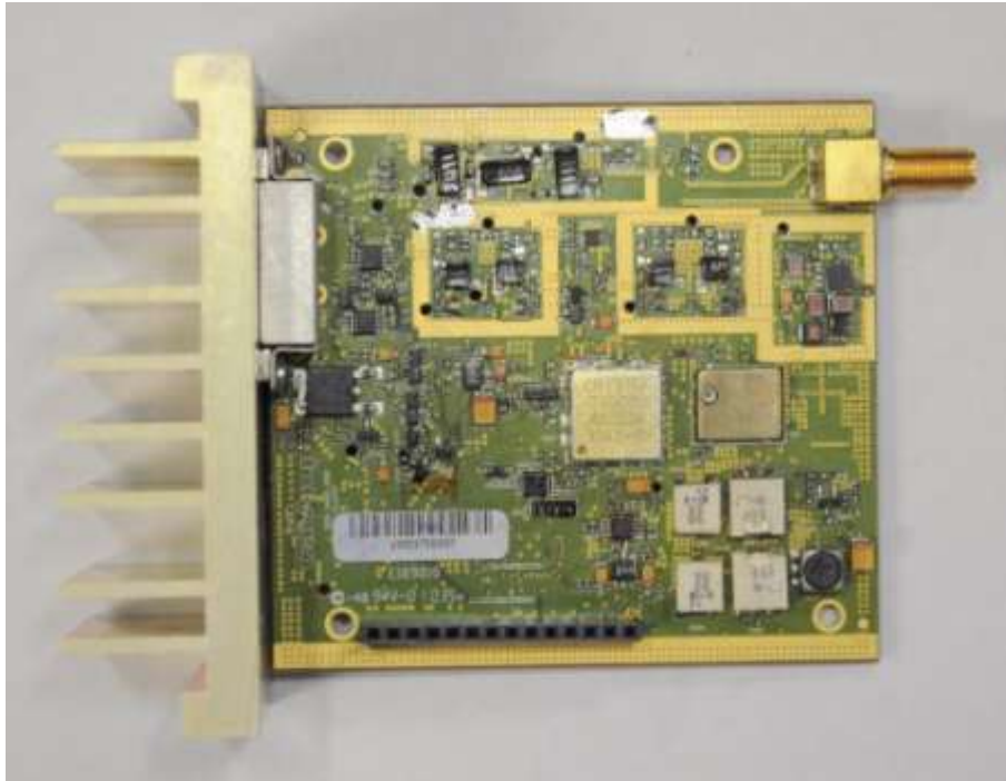
Top Side RF Board no shields
