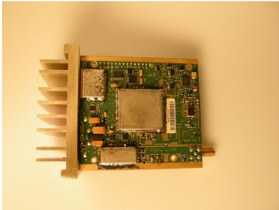
Bottom Side RF Board
