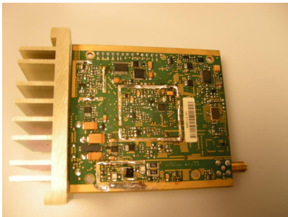
Bottom Side RF Board no shields
