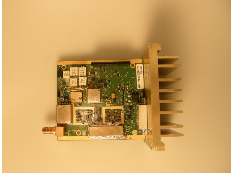
Top Side RF Board
