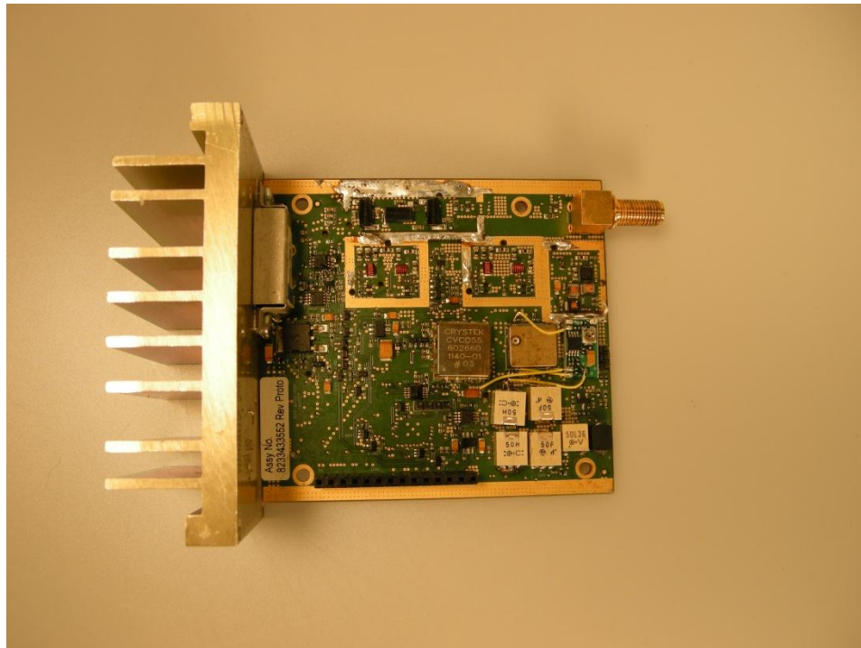
Top Side RF Board no shields
