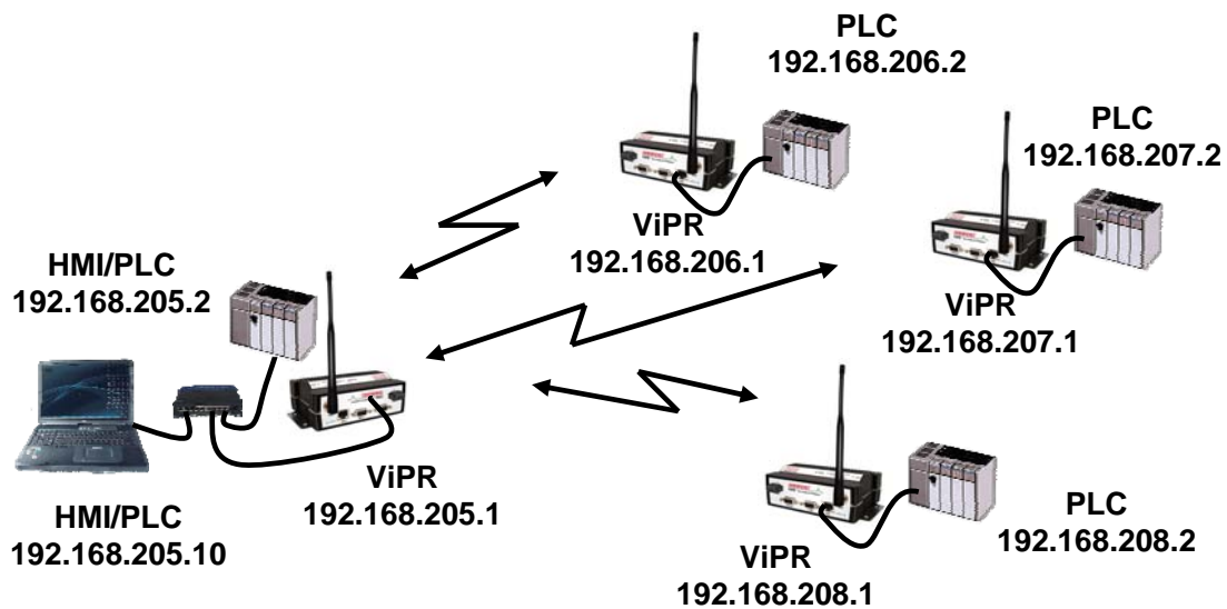
Figure 2.6 ViPR Router Mode Configuration DATARADIO VIPR QUICK START
