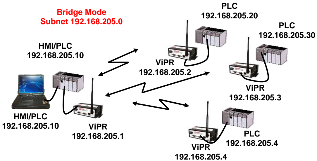
Figure 6.2 ViPR Bridge Mode Configuration.
