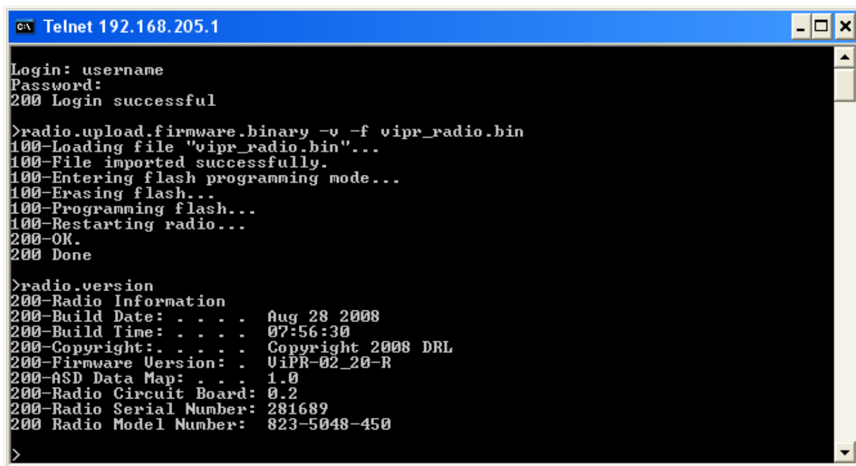
Figure 13.2 Using Windows Command Prompt to upgrade Radio Firmware.
