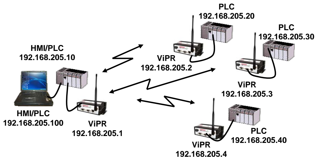
Figure 2.5 ViPR Bridge Mode Configuration
