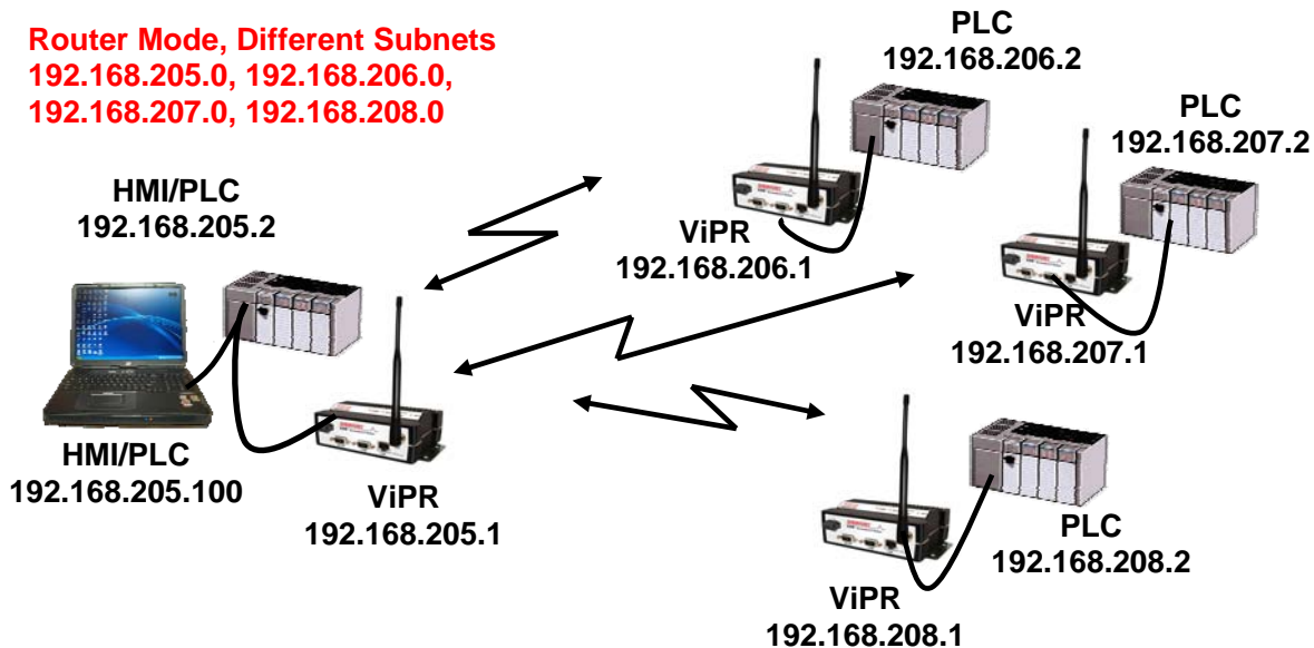
Figure 6.3 ViPR Router Mode Configuration
