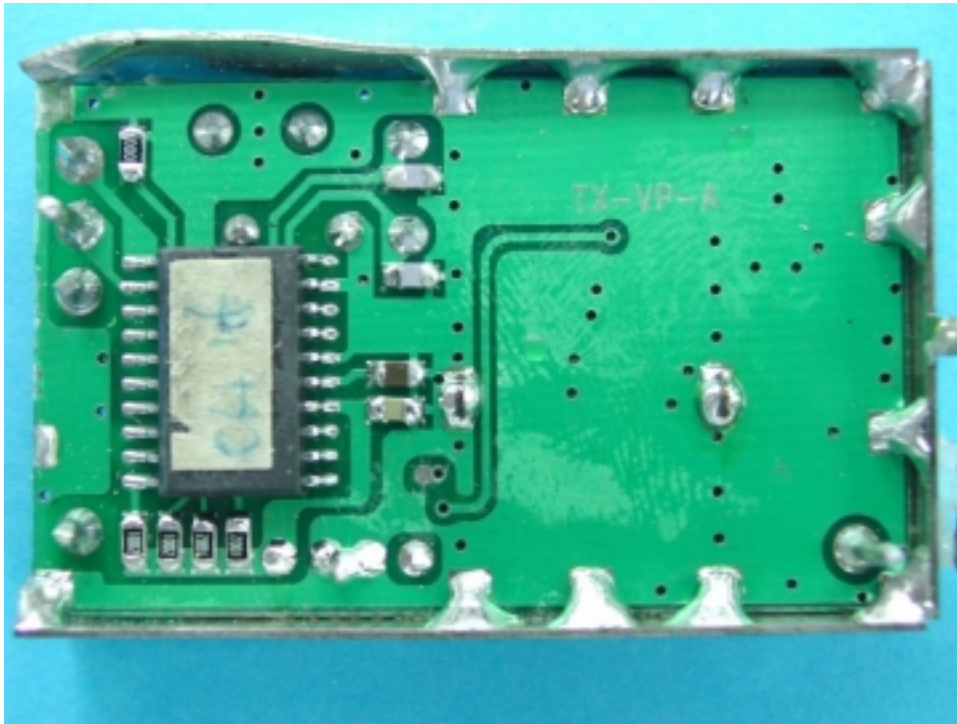
Oscillator PCB solder side
