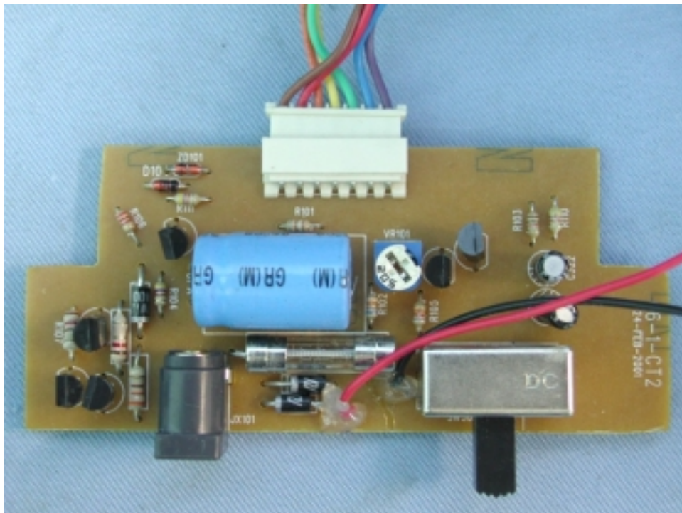
L/L+R/R Selector PCB comp side
