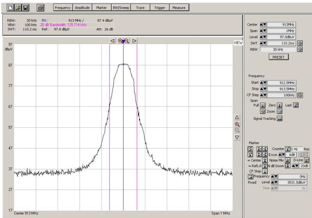
Channel 2 – 20 dB point, Bandwidth 125.7 kHz
