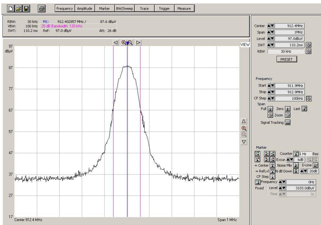
Channel 1 – 20 dB point, Bandwidth 120 kHz
