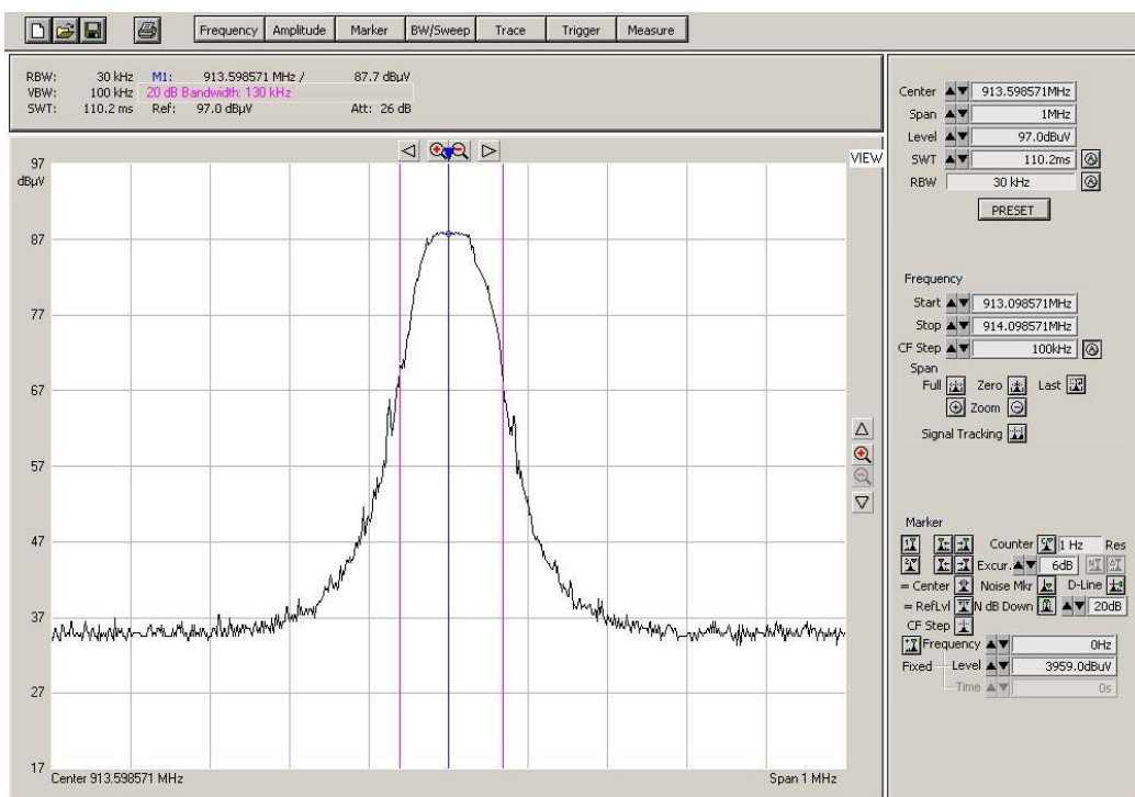
Channel 3 – 20 dB point, Bandwidth 130 kHz
