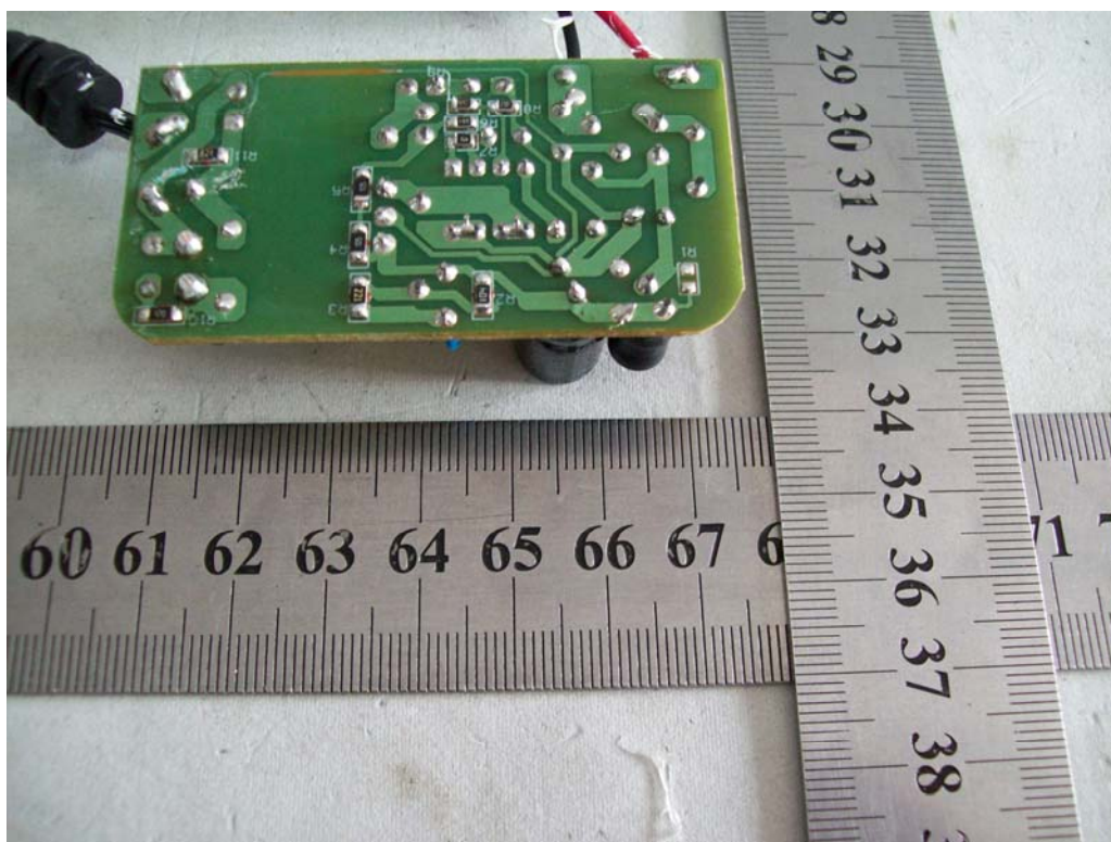
INTERNAL PHOTO OF THE ADAPTER-2
