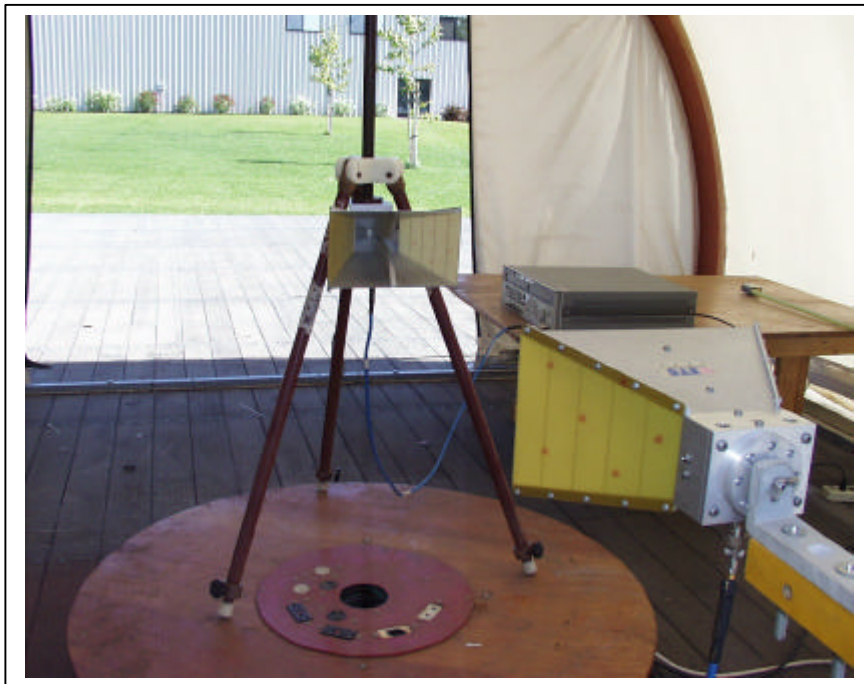
SUBSTITUTION MEASUREMENTS
